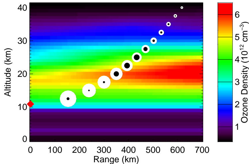
Fig. 2. Integration of the 3-D proxy ozone field. A 2-D curtain plot of ozone number density is oriented along the solar line of sight (SZA=90°, roughly to the south) with the range indicated along the abscissa from a point along the DC-8 flight track on 26 January 2003, (71° N, 25° W) – the same point from which the profiles in Fig. 1 are derived. The DC-8 was at an altitude of 11 km (indicated with a red diamond on the ordinate). Black-on-white solid circles spaced every 2.5 km in the vertical above the DC-8 indicate the path of the line of sight through the atmosphere. The areas of the solid circles are proportional to the ozone absorption contribution function (ozone density \times geometric weighting) in the 2.5-km layer. The white solid circles correspond to the inhomogeneous Case 3 integration of the proxy field. The black, overlying solid circles correspond to the differences between the Case 3 and homogeneous Case 2 (Case 3–Case 2) integrations of the proxy field, the latter assuming a uniform, homogeneous field based on the vertical, 1-D interpolation of the proxy at the DC-8 location. The ozone total slant column density for the Case 3 (Case 2) simulation is 2.31 \times 10^{20} ( 2.07 \times 10^{20} ) \text{cm}^{-2} .
