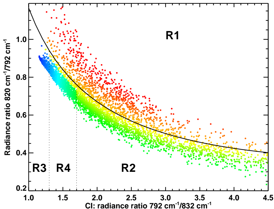
Fig. 1. Mean spectral intensity in the interval 819–821 cm -1 ( I[819\text{--}821\text{ cm}^{-1}] ) divided by I[788.2\text{--}796.25\text{ cm}^{-1}] versus I[788.2\text{--}796.25\text{ cm}^{-1}]/I[832.3\text{--}834.4\text{ cm}^{-1}] of MIPAS PSC observations in May/June 2003 for tangent altitudes between 16 and 25 km. The color scale of the data points denotes their relative position with respect to the different regions in the plot and is used to describe MIPAS measurements and simulations in the following figures.
