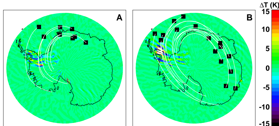
Fig. 4. Color-coded MWF3 hindcast mountain-wave temperature perturbations for 12:00 UT on 10 June (A) and 12:00 UT on 11 June (B) . Overlaid backward trajectories (white lines) start at the times and locations of MIPAS NAT observations (squares) on 11 June (A) and 12 June (B) and end at 00:00 UT on 10 June (A) and 00:00 UT on 11 June (B) . Note that the MWF2 solutions in Fig. 3 show peak wave amplitudes only, whereas the MWF3 runs in this figure provide both amplitude and phase.
