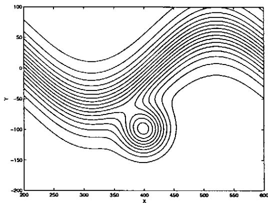
Fig. 9. Streamfunction contours for the strong-eddy case. Snapshots taken at times t = 0 , top; t = 0.16T , middle; t = 0.32T , bottom. Spatial coordinates in km , contour spacing 0.5km^2/min .
