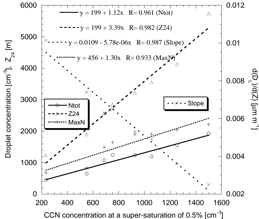
Fig. 9. The relations between CCN concentration at 0.5% SS and four FSSP derived micro-physical parameters: N_{tot} – the average droplet concentration, Z_{24} – the required cloud depth for the onset of warm rain, MaxN – averaged maximum droplet concentration and Slope – the derivative of D_L with height. Each point represents one complete profile, which is based on at least five cloud penetrations at a range of heights of more than 1 km. Clear linear relations between these independent measurements are seen for all variables.
