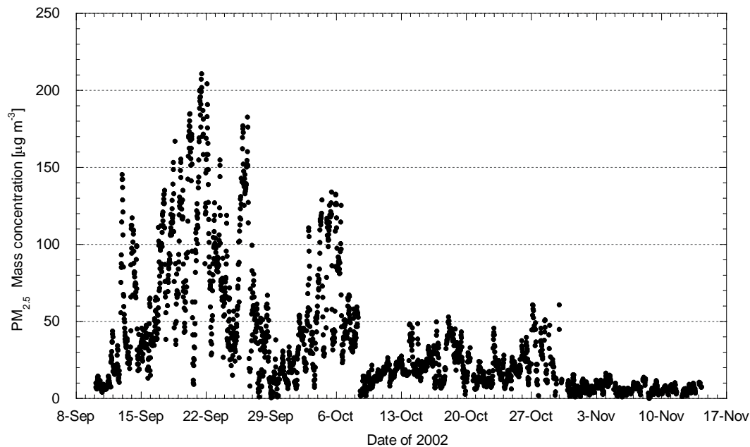
Fig. 1. Half-hour \text{PM}_{2.5} mass concentrations at Fazenda Nossa Senhora (FNS) using a TEOM instrument for the whole period of the LBA-SMOCC field experiment. It can be seen that the entire measuring period can be roughly divided into three sub periods, ending at 8 October, 30 October and 14 November 2002, respectively.
