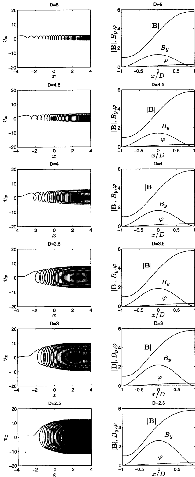
Fig. 1. Trajectory of the electron starting with the velocity \mathbf{v}_0 = (V_u, 0, 0) for different ramp half-widths: 5, 4.5, 4, 3.5, 3, and 2.5 c/\omega_{pe} (top to bottom). The right hand column shows the corresponding field profiles, used for numerical analysis.
