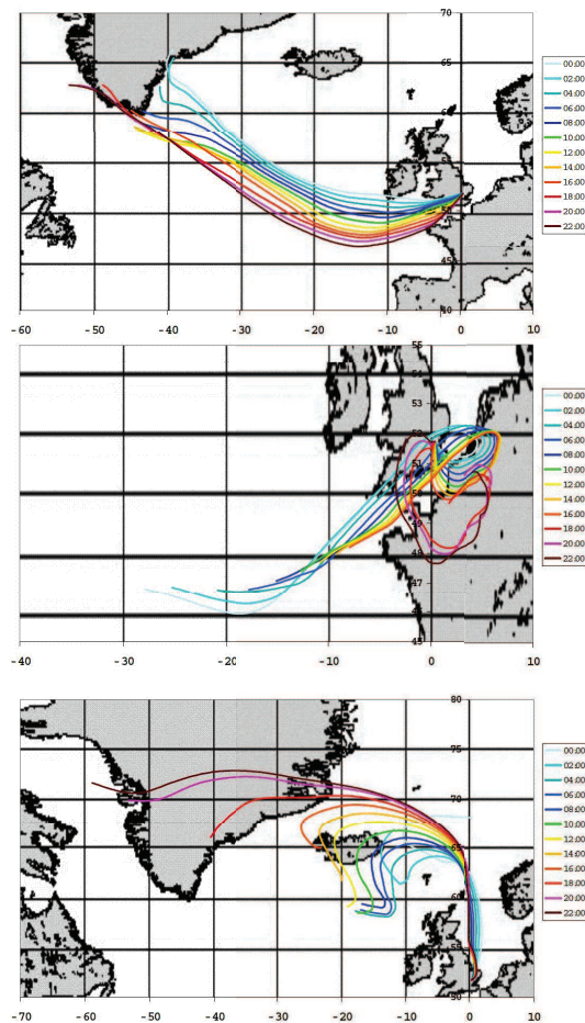
Fig. 2. Representative back trajectories as calculated for the TORCH sampling site by the HYSPLIT model for the Atlantic South Westerly, European Anticyclonic and Arctic Influenced air masses.
