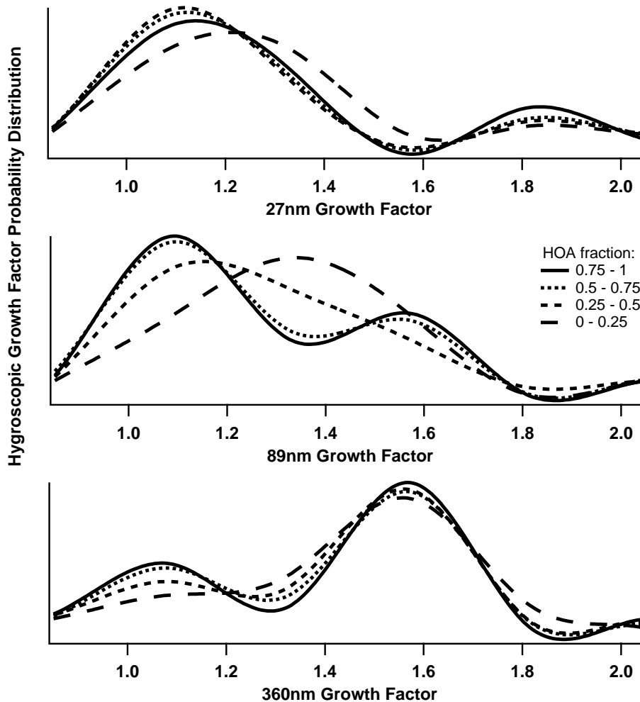
Fig. 11. The transformation of the hygroscopic properties of the ambient aerosol with increasing oxygenated organic content.
