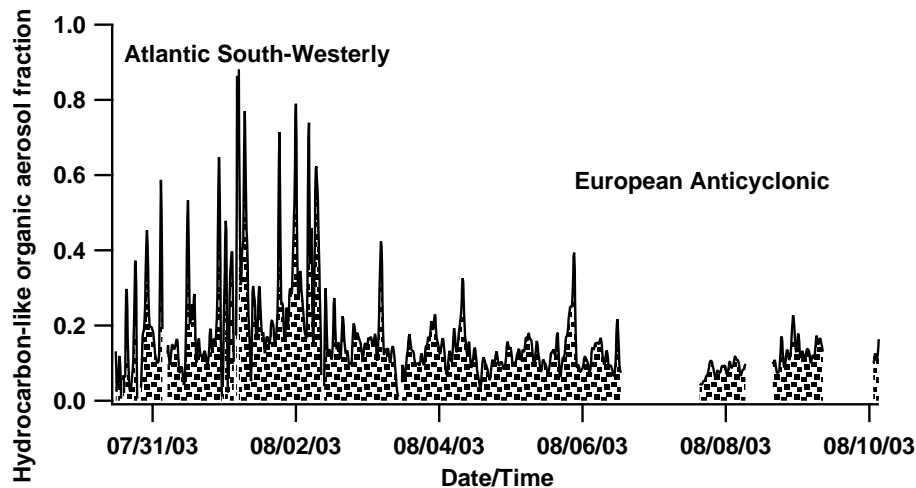
Fig. 8. Time series of the hydrocarbon-like organic aerosol fraction of the total organic content.
