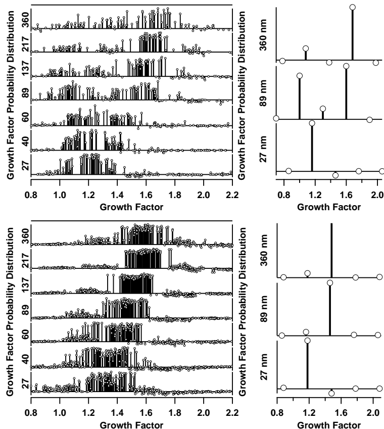
Fig. 5. All the individual (left) and representative individual (right) growth factor distributions for the Atlantic South-Westerly (top) and European Anticyclonic (bottom) periods for different dry particle diameters (indicated on the vertical axes, nm). The cumulative plots show all the retrieved distributions during these periods together, giving an indication of the variability of the modes. The individual plots highlight a single retrieval from one point in time.
