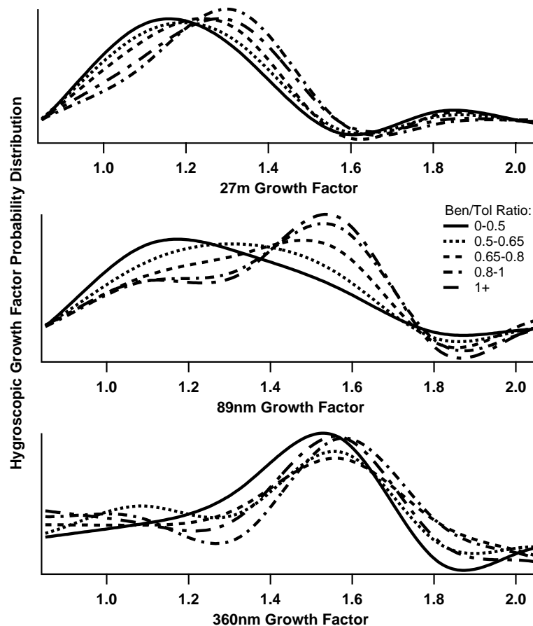
Fig. 9. Mean retrieved hygroscopic growth distributions from the entire TORCH campaign averaged as a function of the VOC ratio benzene/toluene as a marker of photochemical age. Particle dry diameter is indicated on the x-axis.
