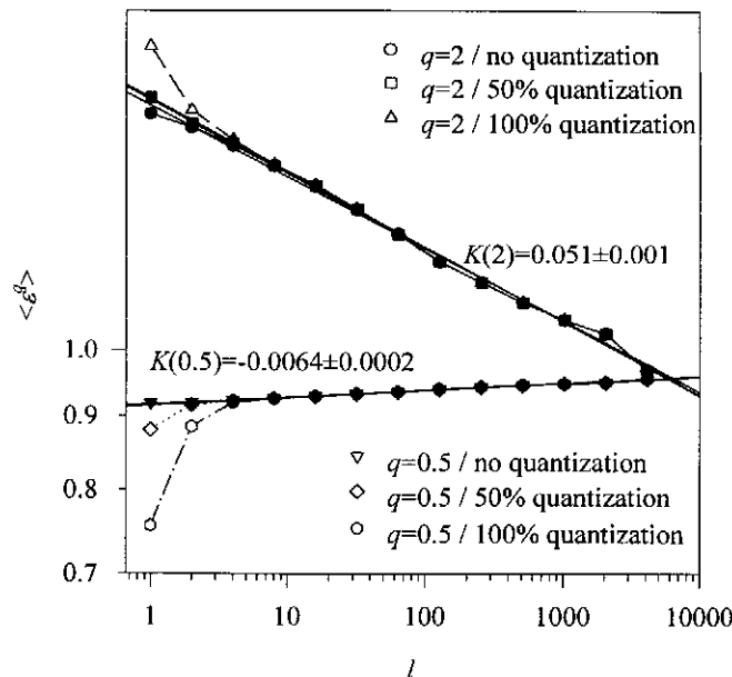
Fig. 13. The effect of quantization on scaling moments.
