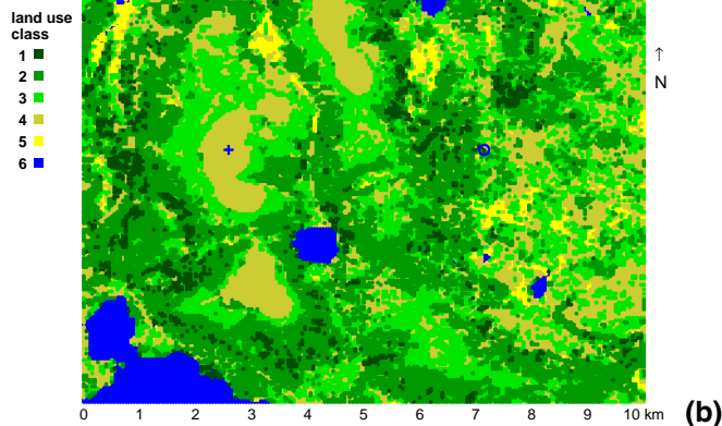
Fig. 1. Topography (a) and land use (b) in the 10×10 km model domain enclosing the Pallas measurement sites. The hill site is marked with a cross and the forest site with a circle.
