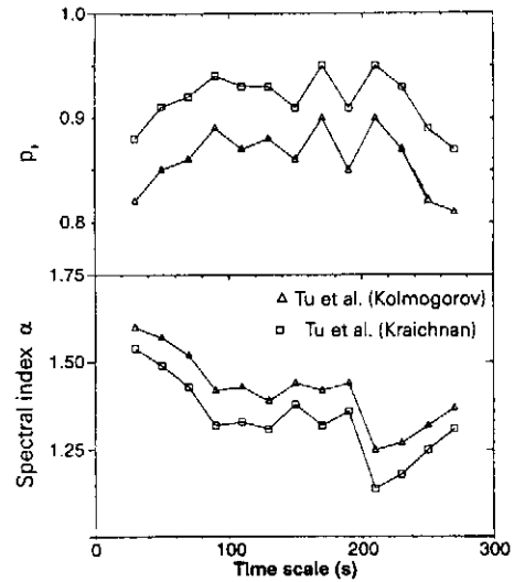
Fig. 13. The scale dependence of the best-fit intermittency parameter P_1 and of the intrinsic spectral index \alpha of the intermittency model by Tu et al. (1996). The parameters are plotted versus time for Ulysses magnetic field data taken in the fast polar solar wind at a distance of 1.9 AU and a heliolatitude of 71^\circ . The boxes correspond to a Kraichnan-type and triangles to a Kolmogorov-type cascade (adapted from Horbury et al., 1996).
