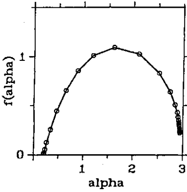
Fig. 16. The multifractal spectrum f(\alpha) plotted versus the singularity exponent \alpha for the data of Figs. 14 and 15 (adapted from Marsch et al., 1996).
