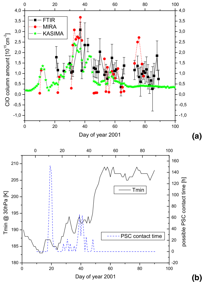
Fig. 4. Time series of column amounts of ClO as measured by FTIR and MIRA and calculated by KASIMA together with possible contact hours with PSCs and the minimum stratospheric temperature (ECMWF data).
