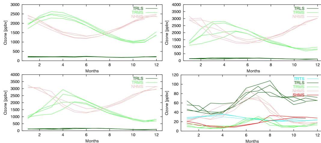
Fig. 5. Seasonal cycle of the ozone mixing ratios (ppbv) from various origin at 60^\circ N and 50 hPa (first row), 90^\circ N and 50 hPa (second row), 90^\circ N equivalent latitude and 50 hPa (third row), and the Equator at 76 hPa (bottom row). Four consecutive cycles are presented.
