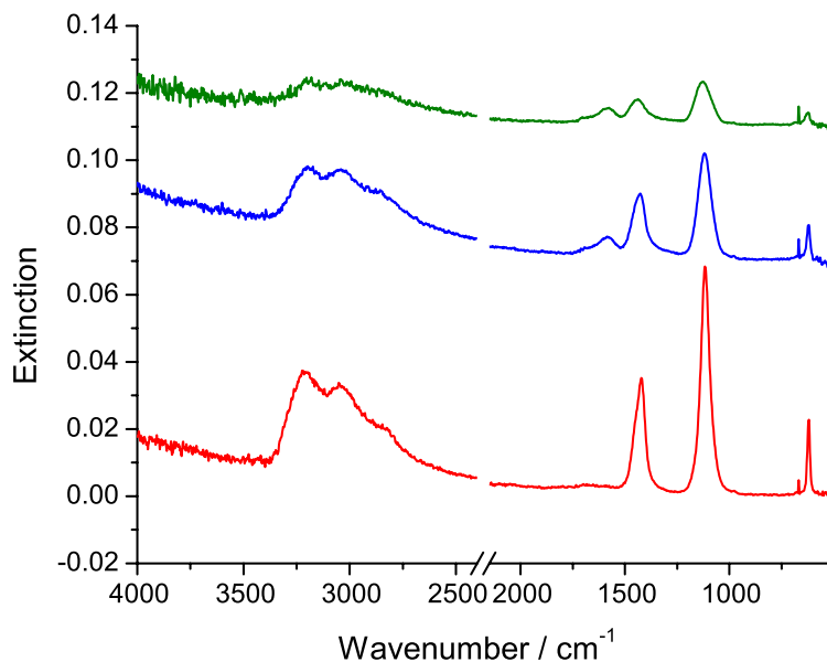
Fig. 7. Dry ( RH \leq 2\% ) IR spectra obtained for aerosols generated from three mixed Aldrich humic acid (NaHA) and ammonium sulphate (AS) solutions. Red line, 1:13 NaHA:AS; blue line, 1:1 NaHA:AS; green line, 1.5:1 NaHA:AS. Spectral features due to CO_2 have been removed. For clarity, gas-phase water lines have been subtracted and the top two spectra off-set by 0.11 and 0.07, respectively.
