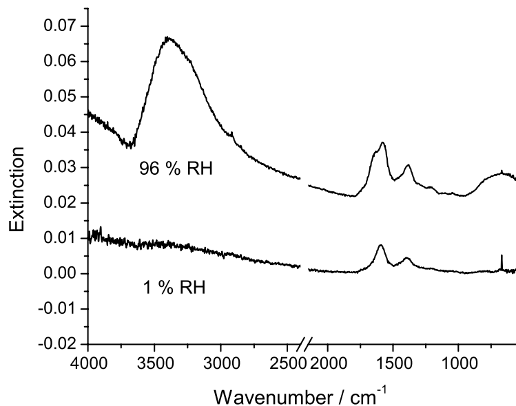
Fig. 5. Infra-red spectra for pH 9 NaHA aerosol obtained during a deliquescence mode experiment. Spectral features due to CO 2 have been removed. Gas-phase water lines have been subtracted and the top spectrum off-set by 0.02 for clarity.
