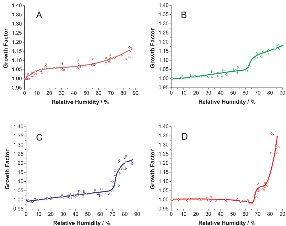
Fig. 10. Growth curves for NaHA (A) , 2:1 NaHA:AS (B) , 1:1.5 NaHA:AS (C) , 1:5 NaHA:AS (D) . Data for both 100 nm (circles) and 50 nm (triangles) diameter particles are shown. The lines act as a guide to the eye.
