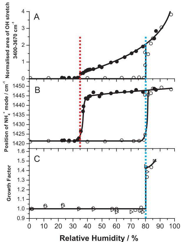
Fig. 3. Water content curve (A) and shifts in \text{NH}_4^+ mode (B) for ammonium sulphate aerosol as obtained using FTIR spectroscopy in both deliquescence (empty circles) and efflorescence modes (filled circles). Growth curve (C) obtained using the TDMA for both 50 nm (circles) and 100 nm (triangles) diameter particles for ammonium sulphate aerosol in deliquescence mode. Dashed blue line, \text{DRH}=80\pm2\% ; dashed red line, \text{ERH}=34\pm2\% . In all cases, the solid lines act as a guide to the eye.
