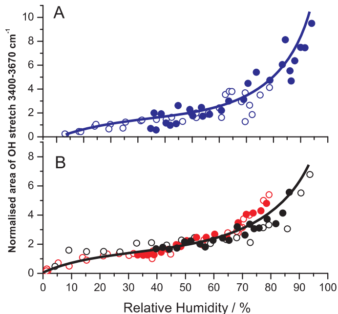
Fig. 6. Water content curves obtained for LSHA (blue symbols), pH 9 NaHA (black symbols) and pH 4 NaHA (red symbols) aerosols. Data are shown for both deliquescence (empty circles) and efflorescence (filled circles) modes. The line acts as a guide to the eye.
