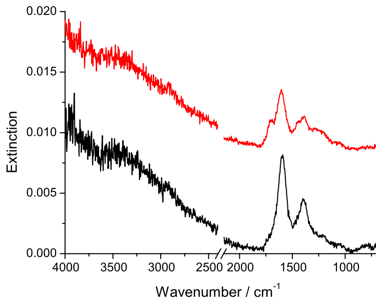
Fig. 4. A comparison of the dry ( RH \leq 2\% ) IR spectra obtained for pH 9 (black line) and pH 4 (red line) NaHA aerosols. Spectral features due to CO_2 have been removed. Gas-phase water lines have been subtracted and the pH 4 spectrum off-set by 0.08 for clarity.
