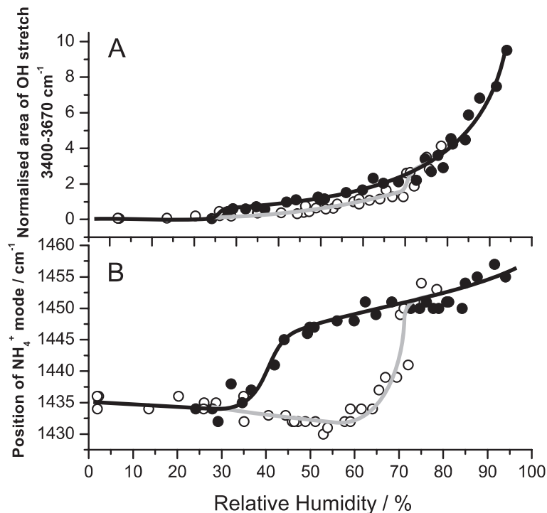
Fig. 9. Water content curve (A) and shifts in \text{NH}_4^+ mode (B) for 1:1 LSHA:AS aerosol in both deliquescence (empty circles) and efflorescence modes (filled circles). The solid lines act as a guide to the eye.
