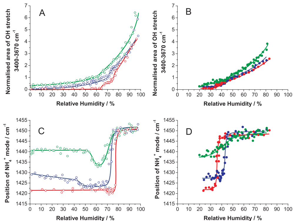
Fig. 8. Water content curves ( A, B ) and shifts in \text{NH}_4^+ mode ( C, D ) for three mixed Aldrich humic acid (NaHA) and ammonium sulphate (AS) aerosols. Red lines, 1:13 NaHA:AS; blue lines, 1:1 NaHA:AS; green lines, 1.5:1 NaHA:AS. Data are shown for both deliquescence (empty circles) and efflorescence (filled circles) modes. The lines act as a guide to the eye.
