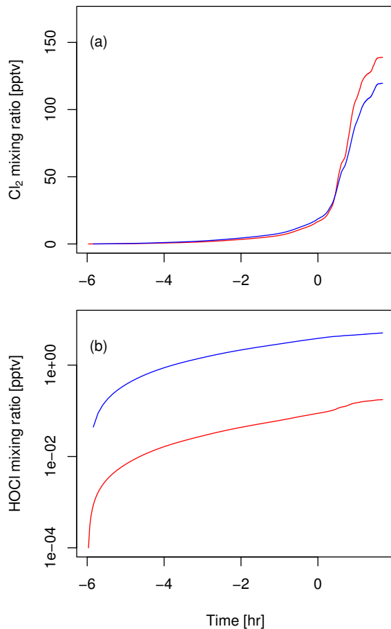
Fig. 12. Production of (a) Cl 2 and (b) HOCl during the T UCSE + 1.5 K model runs shown in Fig. 8. The blue line indicates the output from our microphysical model, the red line that from the equilibrium code.
