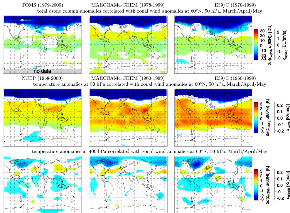
Fig. 7. Similar to previous figures, but showing the size ( 2\sigma ) of anomalies related to Arctic polar vortex strength, for northern spring (March/April/May). Polar vortex strength is represented by zonal wind anomalies at 60° N, 50 hPa.
