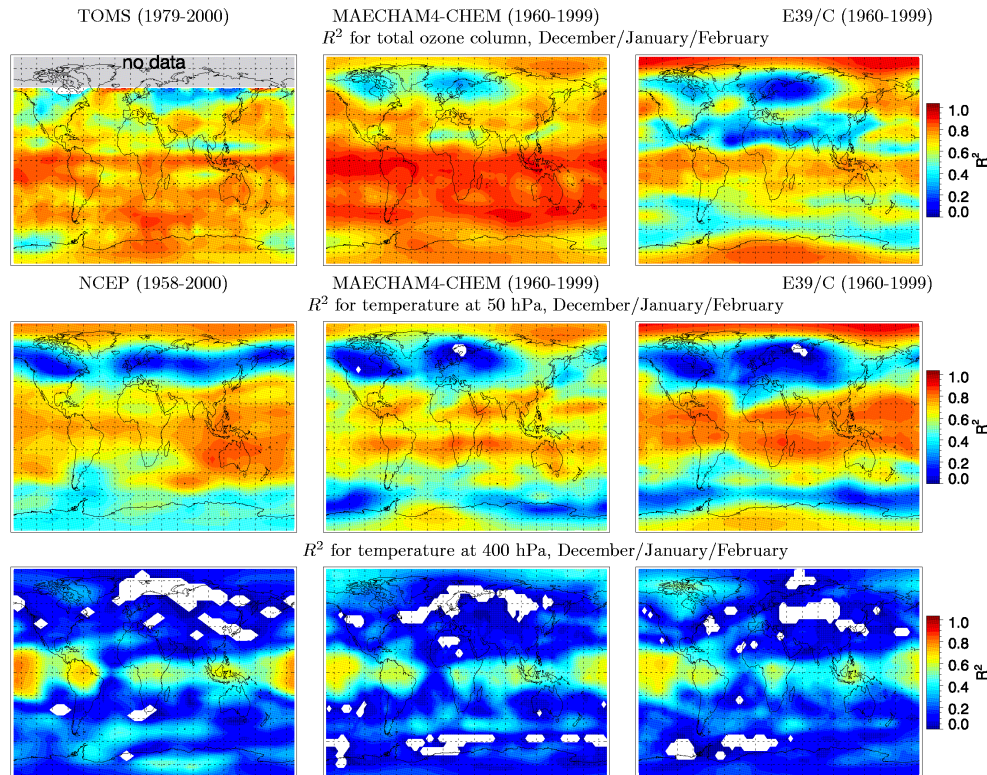
Fig. 2. Global maps of R^2 for northern winter (December/January/February). Top row gives results for total ozone anomalies, middle row results for temperature anomalies at 50 hPa ( \approx 22 km), and bottom row results for temperature anomalies at 400 hPa ( \approx 7 km). R^2 for TOMS/SBUV observations and NCEP reanalyses results is given in the left column, R^2 for the MAECHAM4-CHEM transient simulation in the middle column, and R^2 for the ECHAM4.L39(DLR)/CHEM (=E39/C) transient simulation in the right column. TOMS/SBUV observations are not available before 1979 and are not available in polar regions in winter (grey area).
