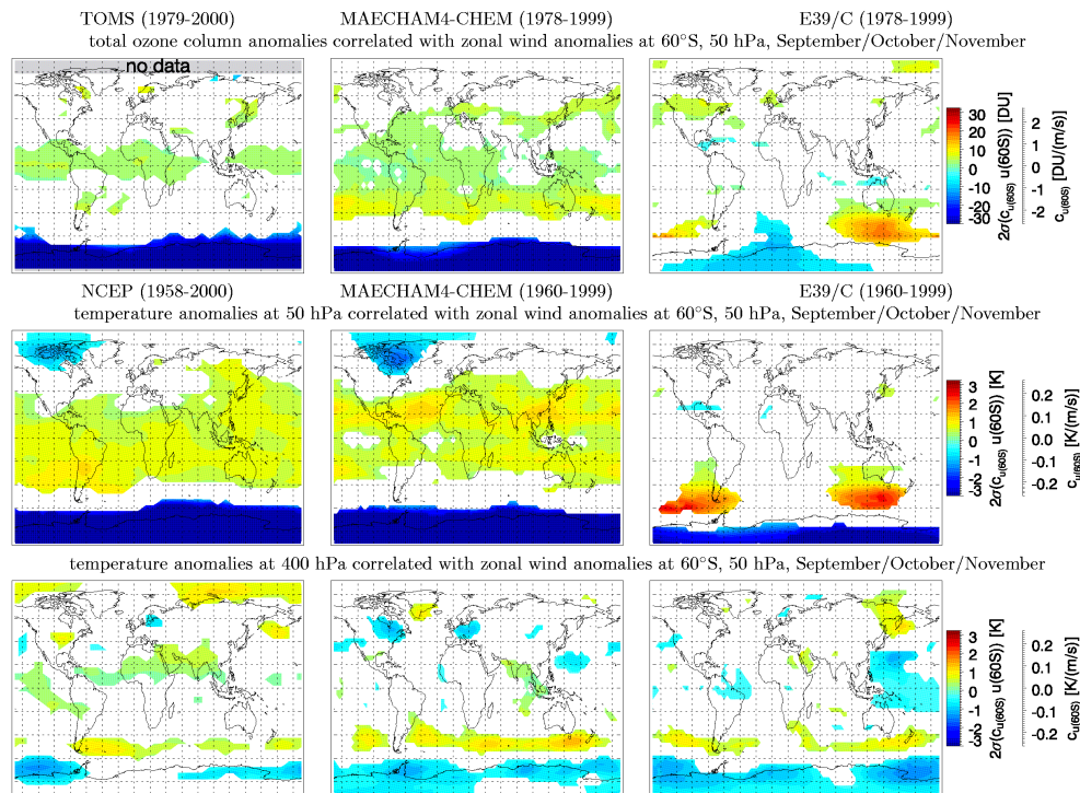
Fig. 8. Same as Fig. 7, but for Antarctic polar vortex strength, and southern spring (September/October/November). Antarctic polar vortex strength is represented by zonal wind anomalies at 60° S, 50 hPa.
