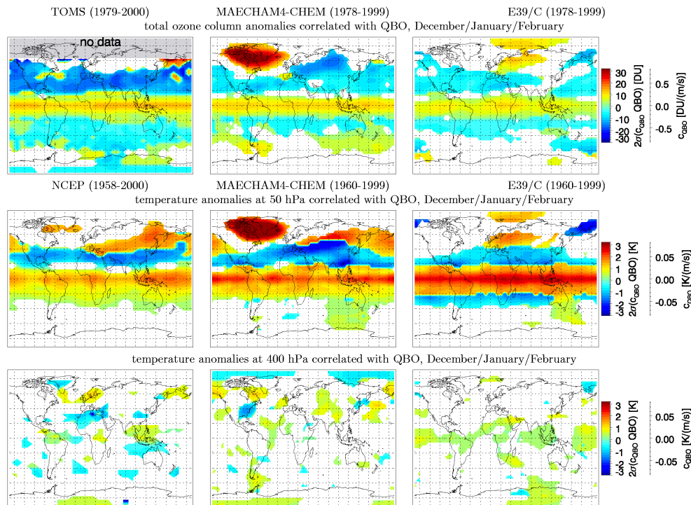
Fig. 4. Similar to previous figure, but showing two standard deviations ( 2\sigma ) of the combined QBO term in the regression, for northern winter (December/January/February). The second scales, on the right, give the approximate size of the QBO regression coefficient \sqrt{c_{QBO(10)}^2 + c_{QBO(30)}^2} . Blue colors indicate inverse (negative) correlation with westerly zonal wind at 30 hPa at the Equator, whereas yellow and red colors indicate positive correlation. For total ozone in the top panels a shorter time period is considered. White regions have no statistically significant QBO-related variation, at the 90% confidence level.
