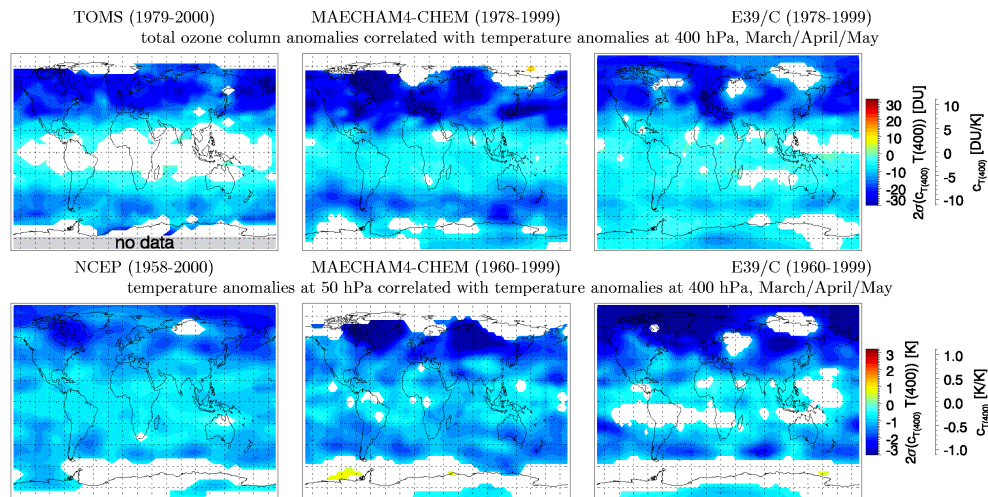
Fig. 9. Similar to previous figures, but showing the size ( 2\sigma ) of stratospheric ozone and 50 hPa temperature anomalies attributed to tropospheric temperature anomalies at 400 hPa (term c_{T(400)} T(400) ). The second scales, on the right, only give the approximate size of the regression coefficient c_{T(400)} .
