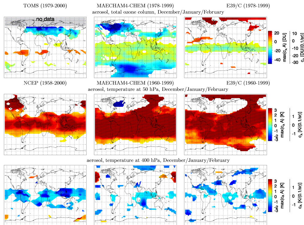
Fig. 6. Similar to previous figures, but for anomalies attributed to stratospheric aerosol from volcanic eruptions, mostly the Mt. Pinatubo eruption. Here the maximum positive or negative anomalies due to the aerosol term ( c_A A ) are shown, not two standard deviations as in the other plots. Red and yellow colors denote positive anomalies, cyan and blue colors negative anomalies. Note that the scale for c_A on the right is only approximate, because aerosol optical density A varies with latitude.
