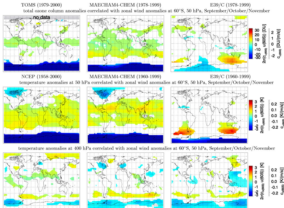
Fig. 8. Same as Fig. 7, but for Antarctic polar vortex strength, and southern spring (September/October/November). Antarctic polar vortex strength is represented by zonal wind anomalies at 60°S, 50 hPa.
