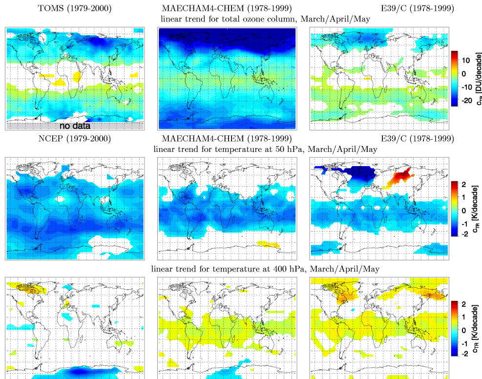
Fig. 3. Similar to previous figure, but showing the linear trend coefficient for northern spring (March/April/May). Top panels give the total ozone trend coefficient in DU per decade, middle and bottom panels give the temperature trend coefficient in K per decade, for 50 hPa ( \approx 22 km) and 400 hPa ( \approx 7 km), respectively. The time period is 1979 to 2000 for observations/reanalysis in the left panels, and is 1978 to 1999 for the model runs in the middle and right panels. In the white regions the linear trend term is not statistically significant at the 90% confidence level.
