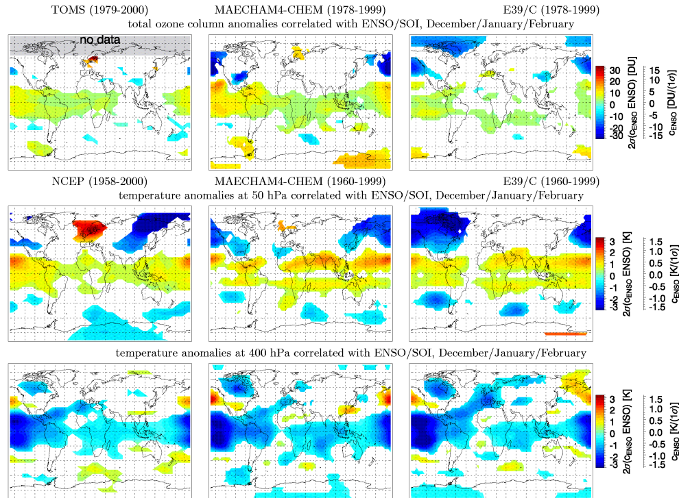
Fig. 10. Same as previous figures, but showing the size ( 2\sigma ) of anomalies correlated with the El Niño Southern-Oscillation Index. These results were obtained without using 400 hPa temperature as an explanatory variable in Eq. (1).
