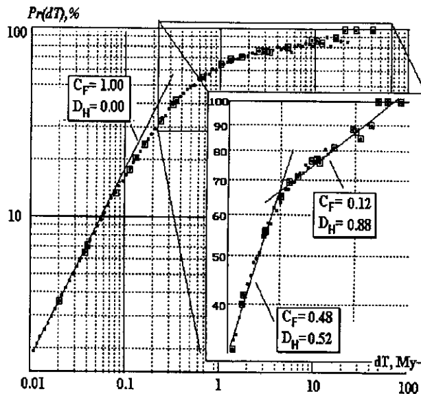
Fig. 3. Dependence of probability of filling of an interval on its duration (box-counting technique). Explanations in text. Inset shows a portion of the graph with exaggerated vertical scale.
