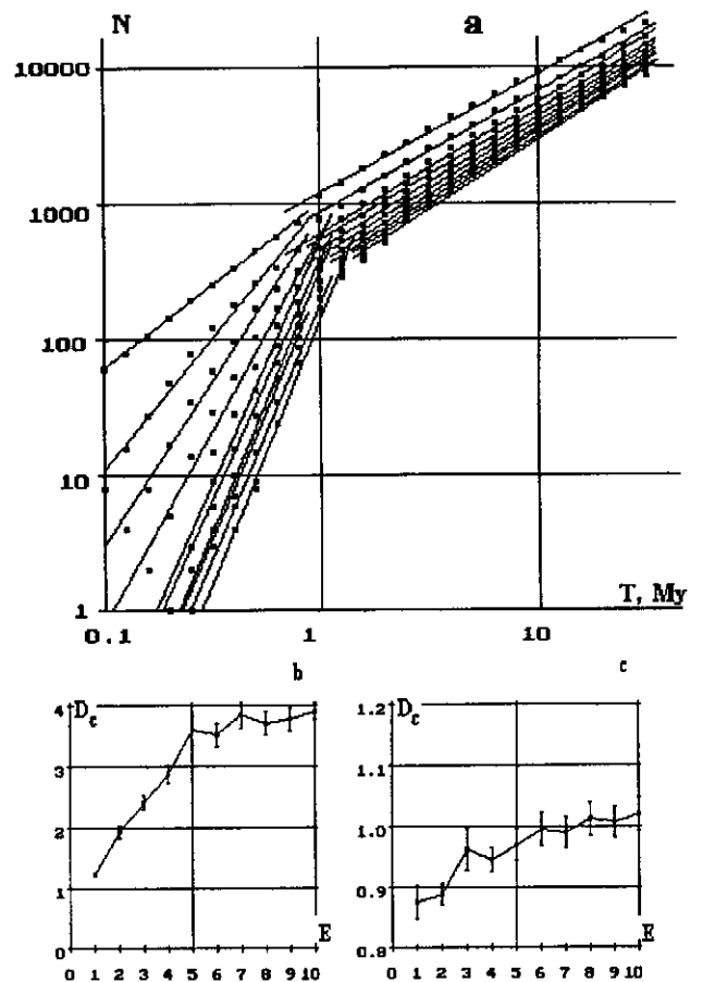
Fig. 6. Results of dimensional analysis of reversal sequence. Graphs of correlation integral vs time span for consequent integer embedding dimensions from 1 (top) to 10 (bottom) with best fit linear approximations (a), and dependence of correlation dimension on dimension of embedding phase space for time spans less (b) and greater (c) than 1 My. Vertical lines - error bars.
