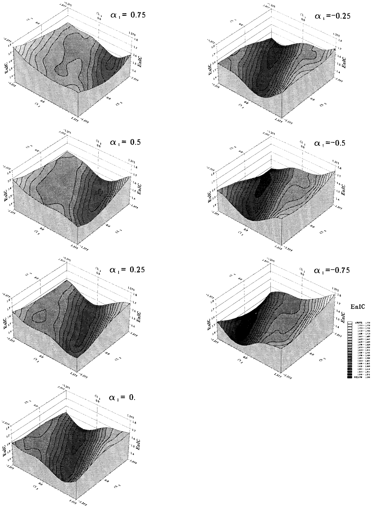
Fig. 3. EnIC for a 3-parameter slowness model
