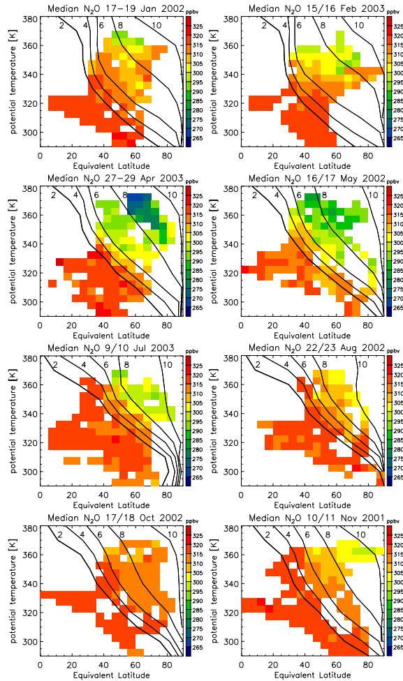
Fig. 3. Same as Fig. 2, but for N 2 O.
