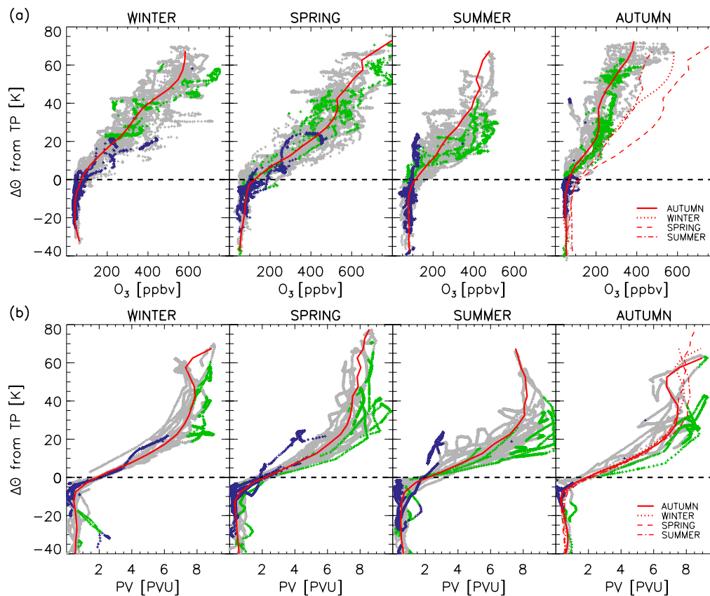
Fig. 7. Same as Fig. 6, but for (a) O 3 and (b) PV.
