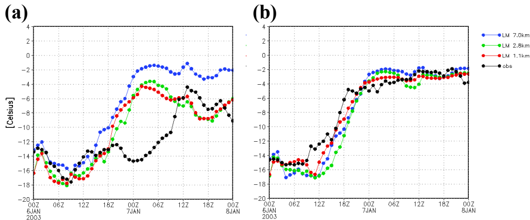
Fig. 10. Time series of 2 m temperature [°C] for LM 7.0 km, 2.8 km, 1.1 km and observations, 48 h forecast of 6 January 2003, 00:00 UTC. (a) Blindern, (b) Tryvann.
