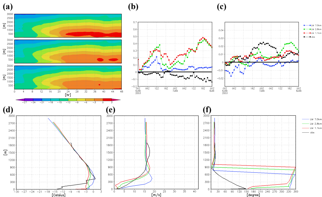
Fig. 11. LM simulations with 7, 2.8 and 1.1 km resolution on 6 January 2003, (a) Blindern, time series of vertical temperature [°C], 48 h forecast starting 00:00 UTC+00 h. Time series of vertical temperature gradient [°C/m] for (b) Hovin and (c) Tryvann/Blindern. Forecasts for 6 January 2003, 00:00 UTC+24 h, vertical LM profiles and radiosoundings at Blindern for (d) temperature [°C], (e) horizontal wind speed [m/s], (f) horizontal wind direction [°].
