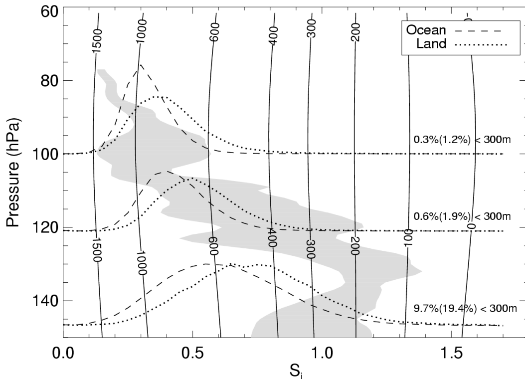
Fig. 7. Distributions of S_i in the tropical TTL retrieved 20^\circ\text{S} and 20^\circ\text{N} using Version 7.02 Microwave Limb Sounder (MLS) measurements aboard the UARS satellite (lines), and in situ from two flights off Honduras flown during the July 2002 CRYSTAL-FACE project (shaded area). Contours represent the estimated isentropic lifting (in meters) required to initiate freezing at that level (Koop et al., 2000). At 146 hPa, assuming deep convection lifts air by 300 m, \sim 20\% ( 10\% ) of land (ocean) air will form pileus cloud. The uncertainty in MLS S_i is approximately 30%, 40% and 50% at 146 hPa, 121 hPa, and 100 hPa, respectively.
