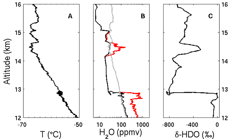
Fig. 3. Profile of (A) temperature, (B) \text{H}_2\text{O} mixing ratios (measured vapour: black; saturation vapour with respect to ice: grey; total (vapour plus ice: red) and \delta\text{-HDO} in a profile obtained on 28 July 2002 over southern Florida. Two isotopically distinct cloud layers are seen: anvil cirrus outflow from convection located below 13 km altitude, and a more tenuous TTL layer centered at 14.5 km altitude. Values of \delta\text{-HDO} in the anvil indicate it originated from lower tropospheric air. In the TTL cloud, values of \delta\text{-HDO} and \text{H}_2\text{O} are intermediate to those in the anvil and TTL. The implication is that the TTC formed from a mixing process between surface and TTL air masses.
