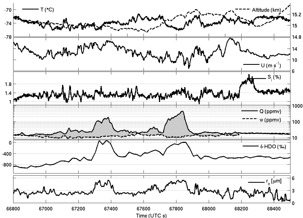
Fig. 4. Flight transect through cloudy air at approximately 15 km altitude off the East coast of Honduras. Measurements show temperature T , altitude, zonal wind velocity U , saturation ratio with respect to ice S_i , total Q and vapor w water mixing ratios, fractionation of HDO relative to H_2O \delta -HDO, and ice crystal effective radius r_e . Shaded area shows mixing ratios of ice.
