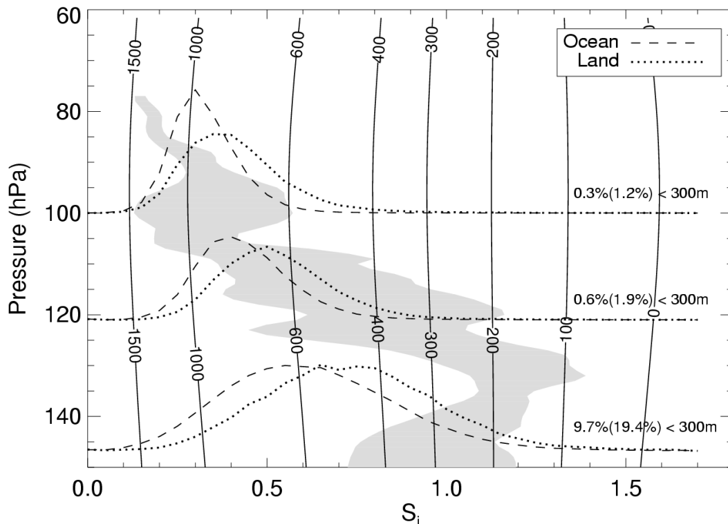
Fig. 7. Distributions of S_i in the tropical TTL retrieved 20^\circ S and 20^\circ N using Version 7.02 Microwave Limb Sounder (MLS) measurements aboard the UARS satellite (lines), and in situ from two flights off Honduras flown during the July 2002 CRYSTAL-FACE project (shaded area). Contours represent the estimated isentropic lifting (in meters) required to initiate freezing at that level (Koop et al., 2000). At 146 hPa, assuming deep convection lifts air by 300 m, \sim 20\% ( 10\% ) of land (ocean) air will form pileus cloud. The uncertainty in MLS S_i is approximately 30%, 40% and 50% at 146 hPa, 121 hPa, and 100 hPa, respectively.
