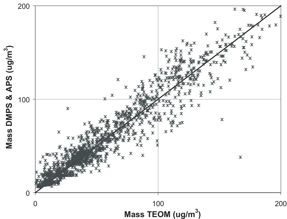
Fig. 2. Correlation plot of the PM_{2.5} measured by the TEOM and the PM_{2.5} calculated from DMPS and APS measurements, using a dry density of 1.37 \text{ g} , for the dry period.
