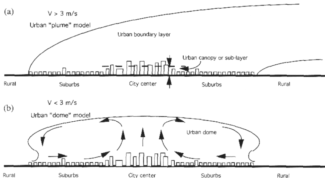
Fig. 6. Meso-scale features which may be present within an urban area. These show possible effects of advection which complicate considerably the “simple” picture shown in earlier figures (after Z. Janour, private communication).
