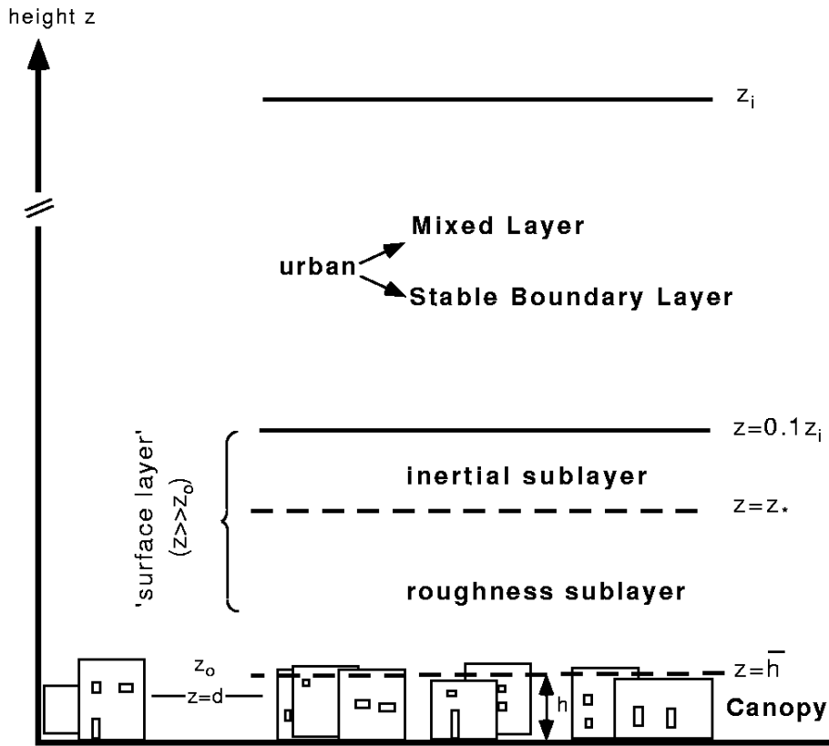
Fig. 3. Idealised structure within the equilibrium urban boundary layer in which typical heights are sketched. \bar{h} denotes the mean height of buildings denoted by z_H in the text.
