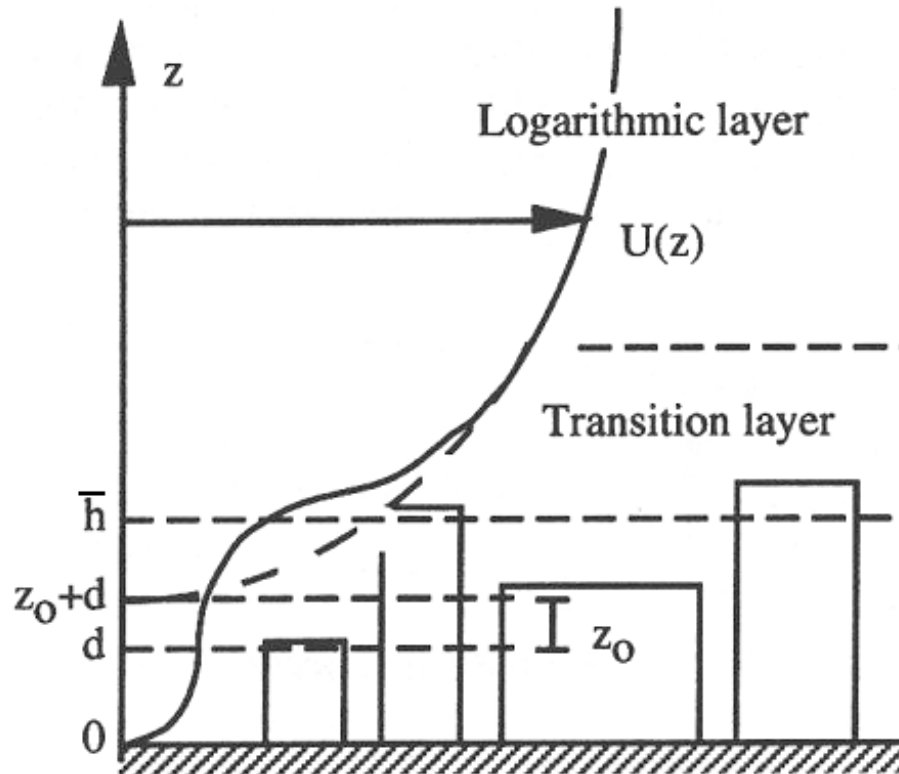
Fig. 4. Sketch of profile within the urban boundary layer. \bar{h} denotes the mean height of buildings denoted by z_H in the text.
