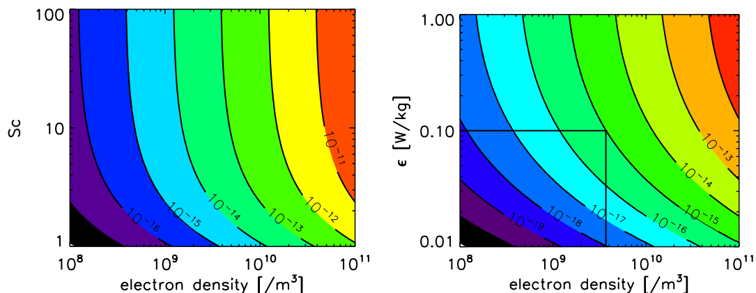
Fig. 8. Left panel: The sensitivity of the volume reflectivity at 3 m to changes in electron density and Schmidt number for \epsilon=0.1 W/kg and N_\theta=1\cdot 10^{-5} /s. Right panel: Same, but for electron density and turbulent energy dissipation rate ( Sc=1 ; N_\theta=1\cdot 10^{-5} /s). A kinematic viscosity of \nu=0.245 m 2 /s is used, representative for an altitude of 70 km.
