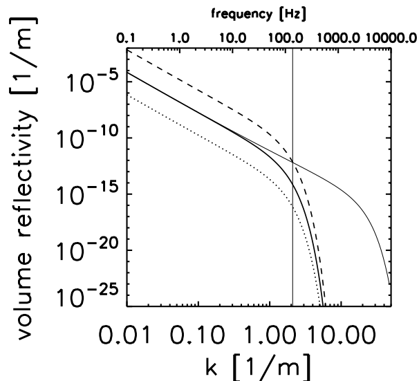
Fig. 6. Volume reflectivity as a function of wave number for various cases of electron densities N_e , Schmidt number Sc , and N_\theta . Standard case (thick solid curve): N_e = 1 \cdot 10^{10}/\text{m}^3 , N_\theta = 1 \cdot 10^{-5}/\text{s} , and Sc = 1 . Relative to the standard case the electron density has been decreased by a factor of 10 (dotted line), N_\theta has been increased by the factor of 100 (dashed line), and the Schmidt number has been increased by a factor of 100 (thin solid line). The energy dissipation rates is \epsilon = 0.1 \text{ W/kg} and the kinematic viscosity is \nu = 0.245 \text{ m}^2/\text{s} for all curves. The value for \nu is representative for an altitude of 70 km. The thin vertical line corresponds to the Bragg scale of the ALWIN radar.
