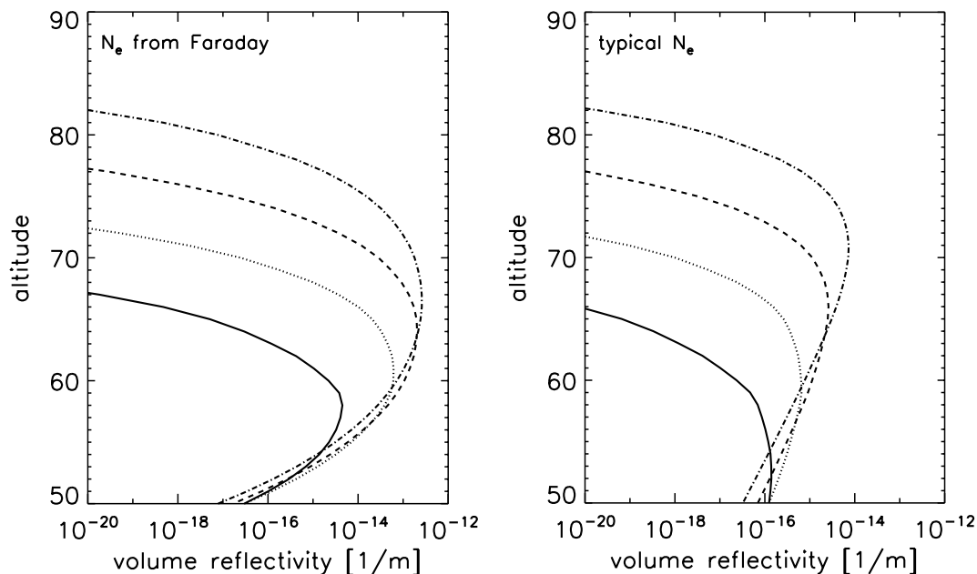
Fig. 10. Left panel: Volume reflectivity at the ALWIN radar Bragg scale for various turbulence strength, namely \epsilon=0.001 (solid), =0.01 (dotted), =0.1 (dashed), and 1 (dashed-dotted). All values in W/kg. The electron density profile from the extended Faraday profile in Fig. 9 has been used. Right panel: Same as left panel but with ‘typical’ electron profile from Fig. 9. For all profiles we have used N_0=1\cdot 10^{-5}/s .
