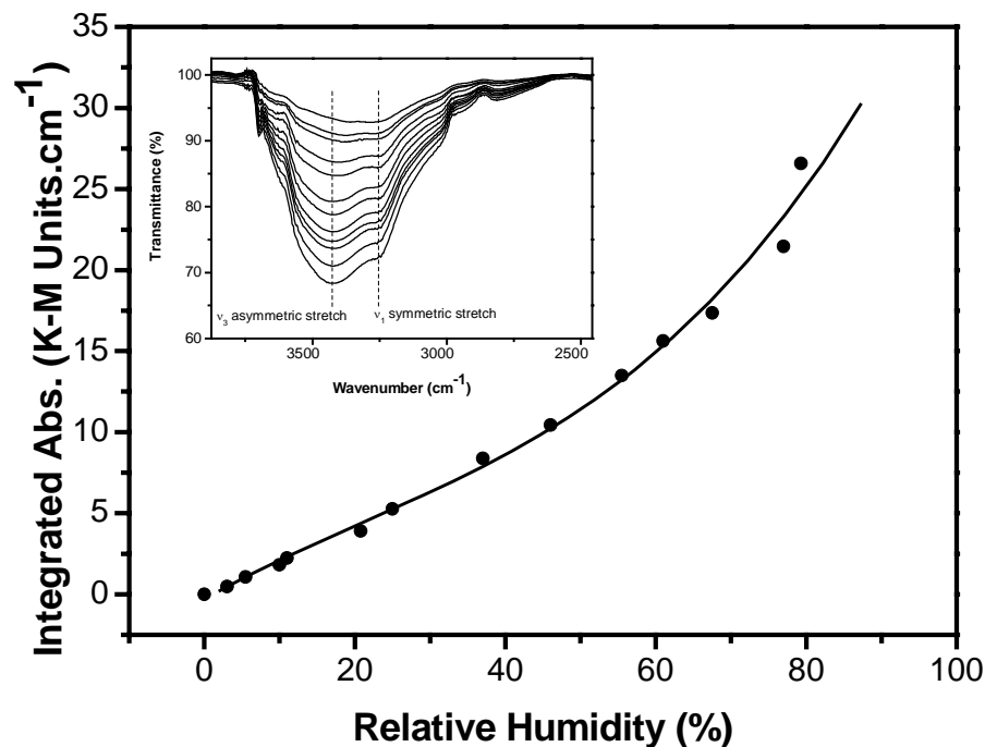
Fig. 1. Water uptake isotherm for calcite obtained using DRIFTS. Region integrated is shown in the inset.
