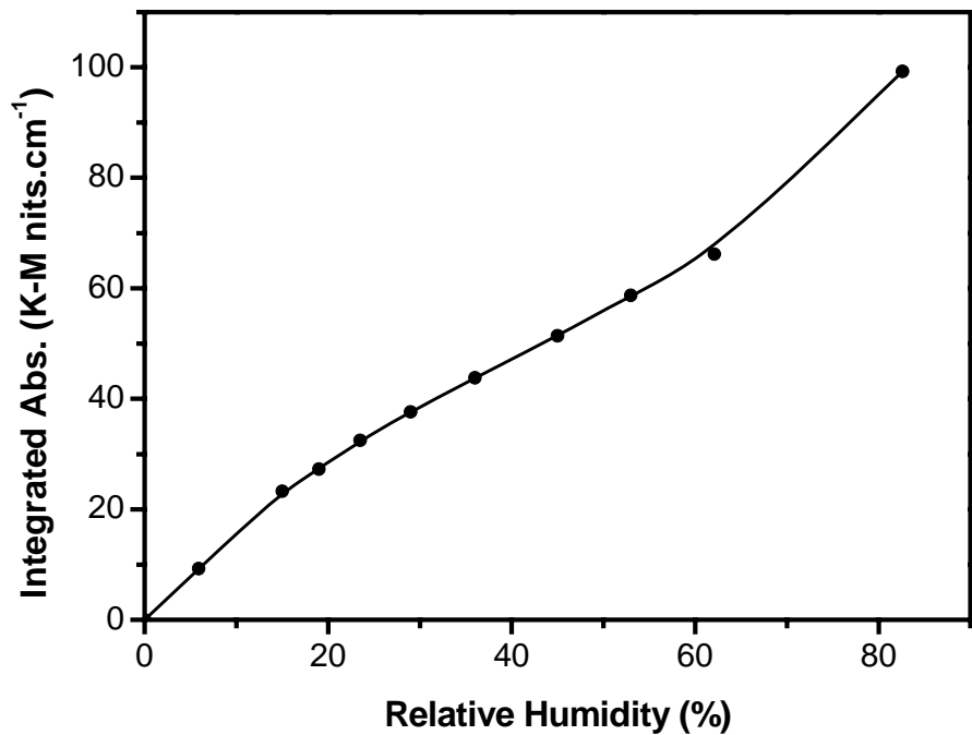
Fig. 5. Water uptake isotherm for ATD obtained using DRIFTS.
