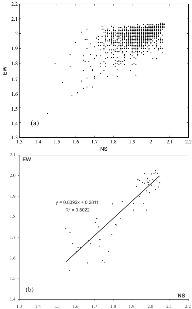
Fig. 9. (a) The scatter plot between NS vs. EW Higuchi exponent along the year. (b) The scatter plot between the same signals but just for data corresponding to the \beta anomaly.
