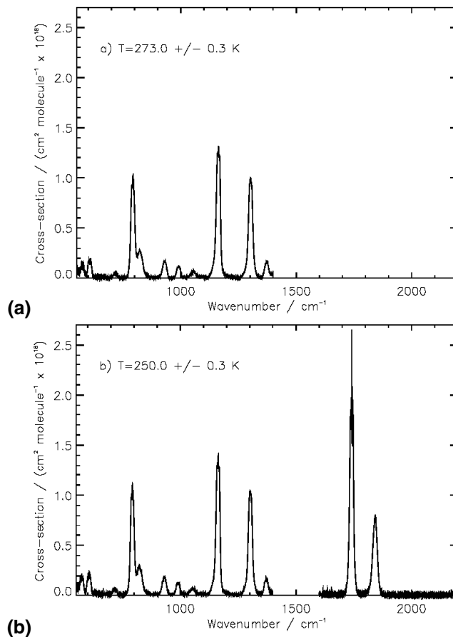
Fig. 1. PAN mid-infrared absorption cross-sections ( 0.25 \text{ cm}^{-1} resolution) at sample temperatures of: (a) 273 \text{ K} \pm 0.3 \text{ K} ( 550 to 1400 \text{ cm}^{-1} ); and (b) 250 \pm 0.3 \text{ K} ( 550 – 1400 \text{ cm}^{-1} , 1600 – 2000 \text{ cm}^{-1} ).
