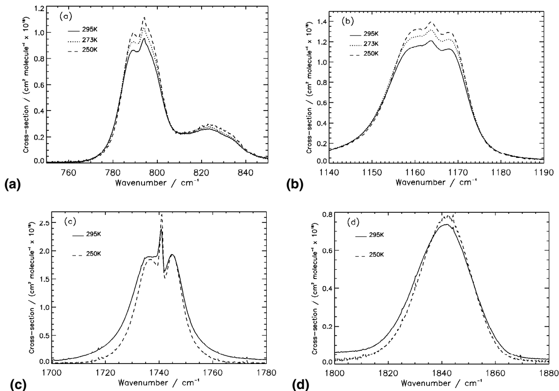
Fig. 2. A close up of the: (a) 794, (b) 1163, (c) 1741 and (d) 1842 \text{cm}^{-1} PAN bands showing temperature dependence at 295 K (solid line) 273 K (dotted line) and 250 K (dashed line). Note: 295 K data taken from Allen et al. (2005) .
