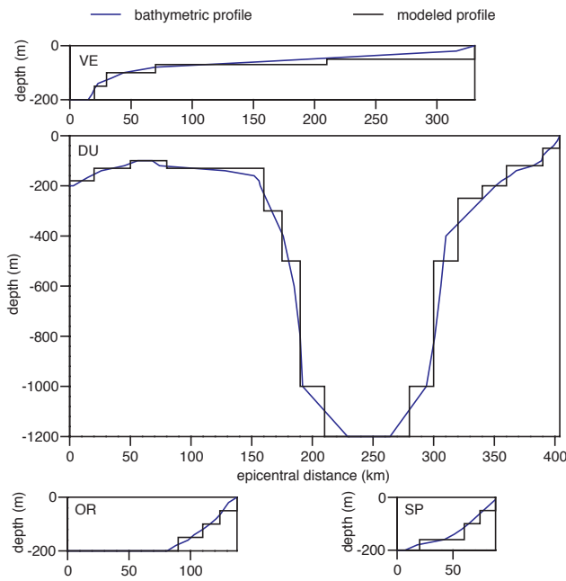
Fig. 2. Bathymetric profiles (in blue) along source-site paths and their parameterisations (in black) used for calculations for the four sites of Zone 1. From above: Venice (VE), Durres (DU), Ortona (OR) and Split (SP).
