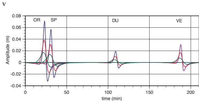
Fig. 3. Synthetic mareograms for Zone 1. Focal depth, H=10 km (blue), 15 km (red), 25 km (green). Magnitude: M=6.5 .
