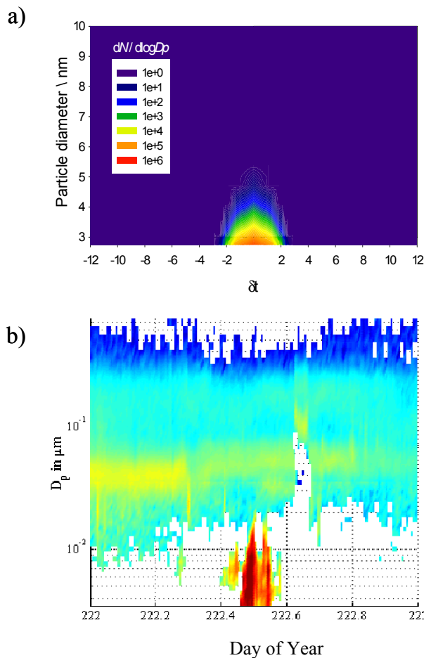
Fig. 10. (a) model simulation of the particle size distribution during a noon low tide particle burst. (b) size distribution measurements on DOY 222, 10th August, as measured by the DMPS instrument.
