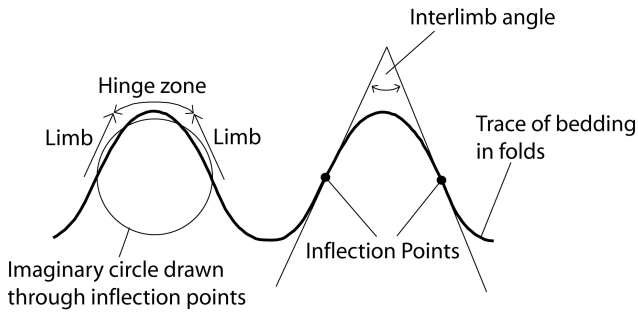
Fig. 3. Diagram showing cross-section view of fold hinge zone, limbs, and interlimb angle. Interlimb angle is the angle formed between lines tangent to the inflection points. Modified after Price and Cosgrove (1990) and Fleuty (1964).
