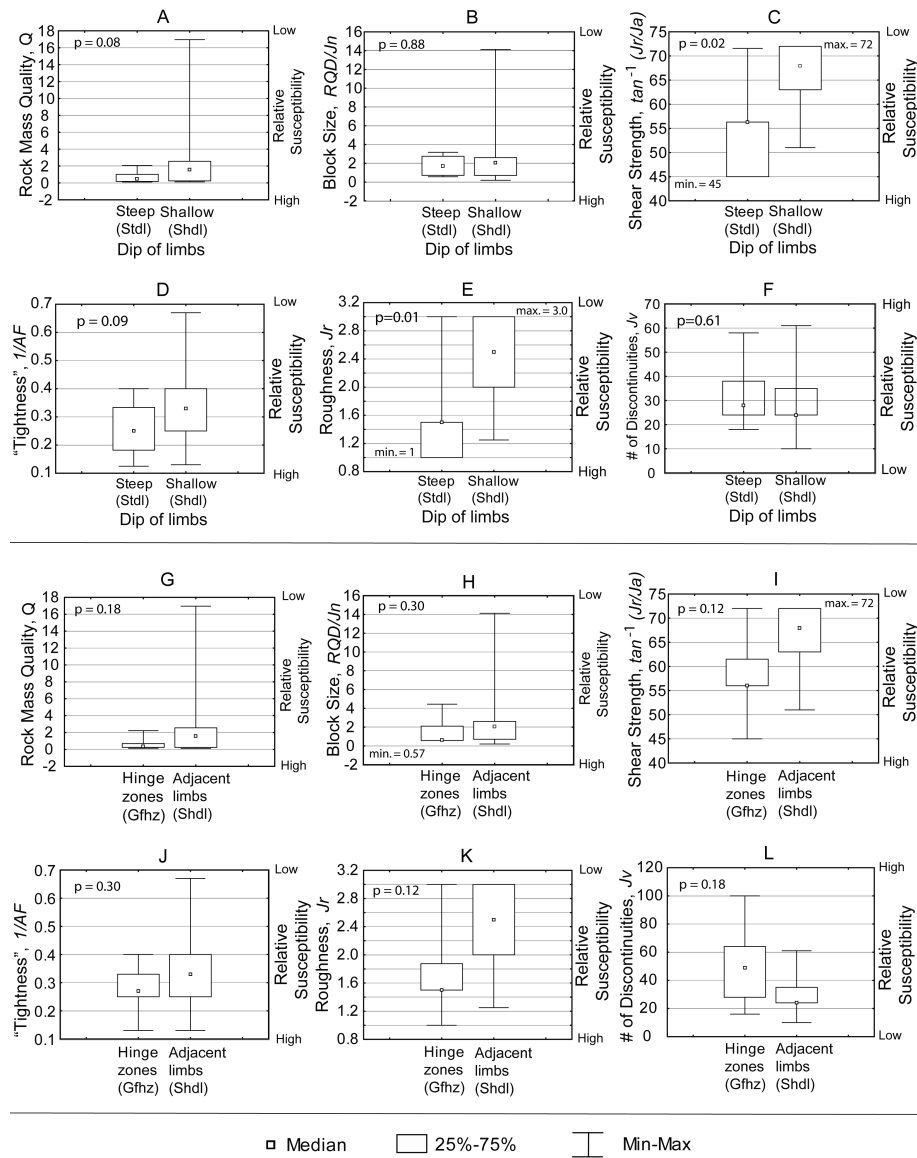
Fig. 8. Box and whisker plots of Q and discontinuity data from the study area. Upper half of diagram contains data from limbs; number of sites is 13 for steep limbs and 13 for shallow limbs; quantity of data from moderate limbs was insufficient (Fig. 2) for statistical analysis. Lower half of diagram contains data from the hinge zone of a gentle fold and adjacent, shallowly-dipping limbs; number of sites is 8 for hinge zones and 13 for adjacent limbs. P values shown are two-tailed values from the unpaired Mann-Whitney statistical analysis.
