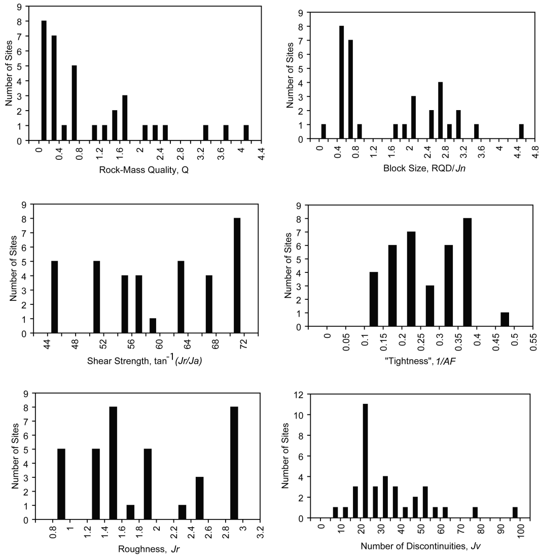
Fig. 6. Histograms showing Q and discontinuity data (see Eq. 1 in text) from the 36 Q measurement sites shown in Fig. 2. Histograms for Q, block size, and “tightness” have 2, 3, and 1, sites, respectively, with values greater than the maximum values shown on the x-axis.
