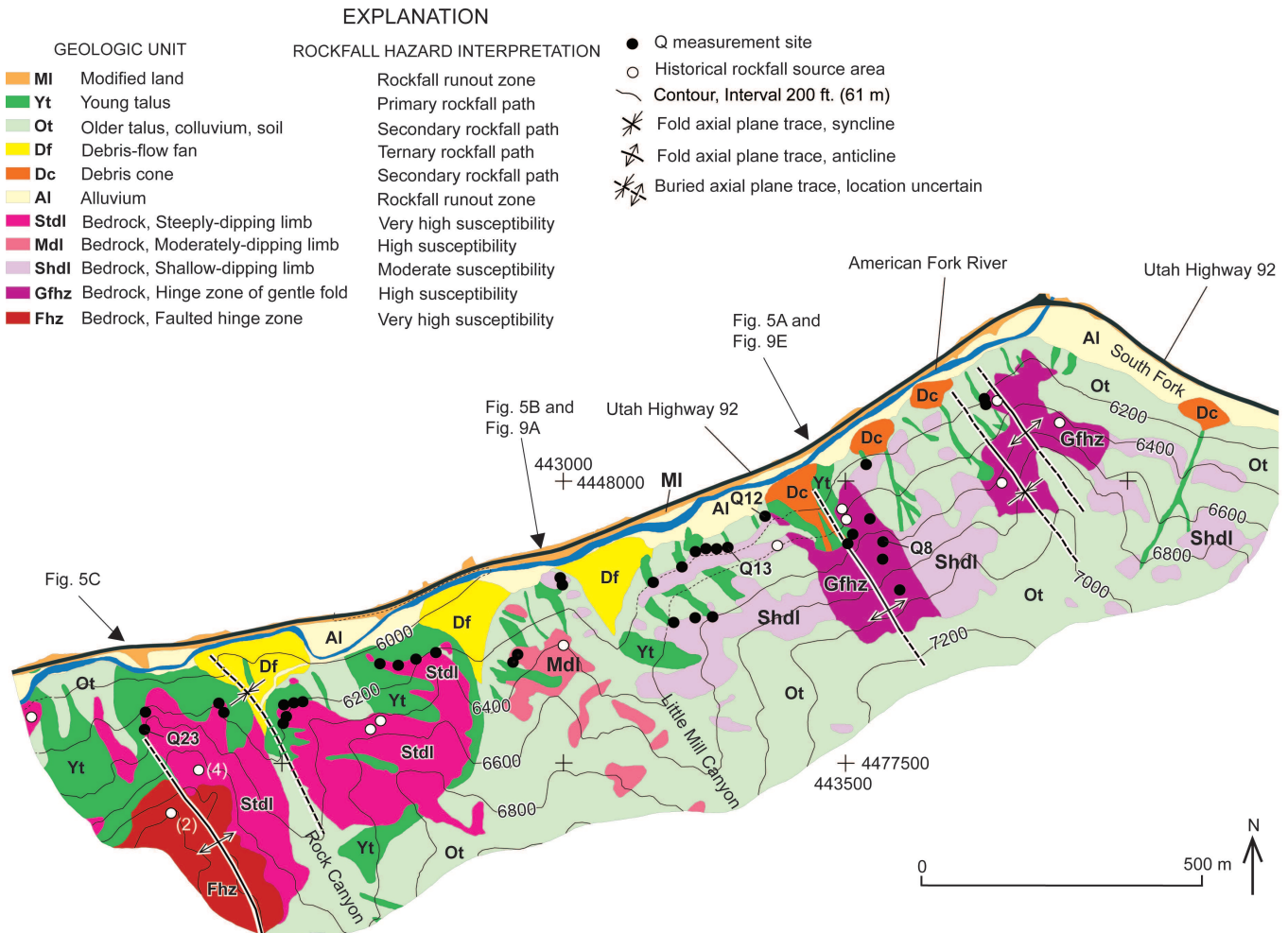
Fig. 2. Geologic map of the study area. Coordinates and tick marks are Universal Transverse Mercator, zone 12N, meters. Fold limbs are defined as follows: shallow dipping, 0-20^\circ ; moderately dipping, 20-40^\circ ; steeply-dipping, >40^\circ . Historical rockfalls are approximately located. Numbers by two rockfalls refer to minimum quantities of falls at those locations.
