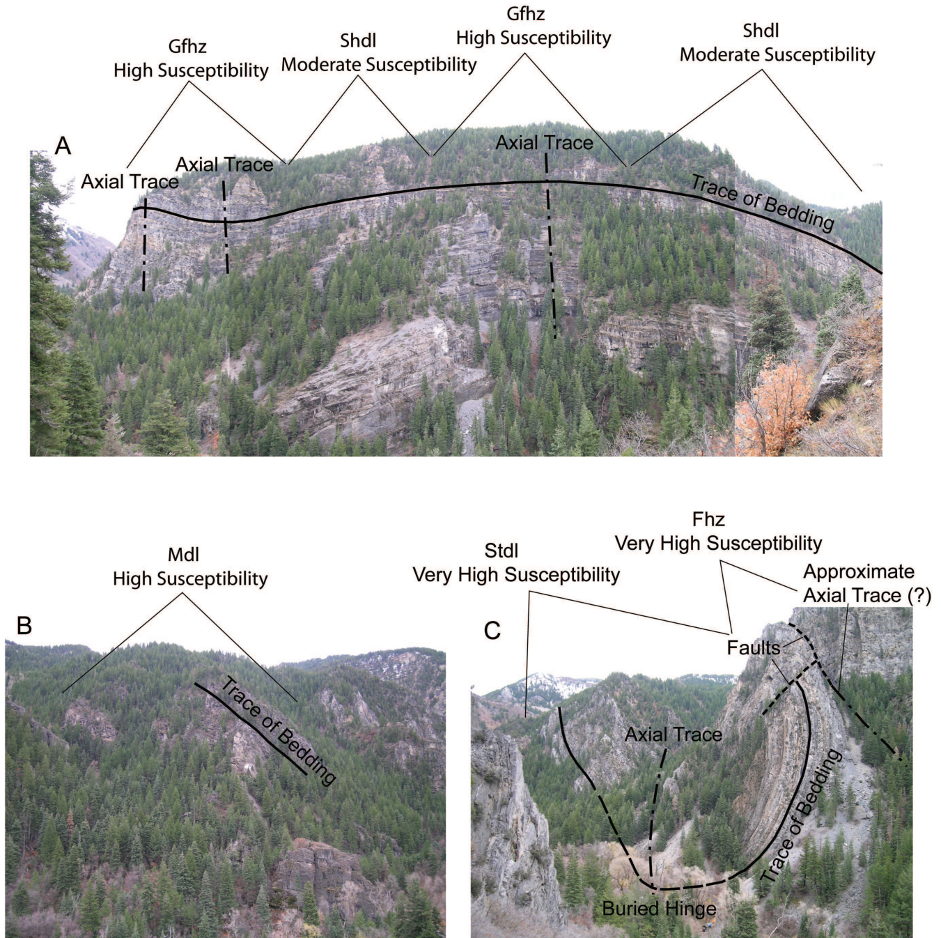
Fig. 5. Folds within the study area as progressing from east (A) to west (C). Solid black lines (dashed where buried) show form of folds. (A) Photo composite showing gentle folds in the eastern (left) and central (right) parts of the study area. Distance across the field of view is about 1500 m. (B) Moderately dipping fold limb in the central part of the study area. Distance across the field of view is about 100 m. (C) Close (buried hinge) and faulted folds in the western part of the study area. Distance across the field of view is about 400 m.
