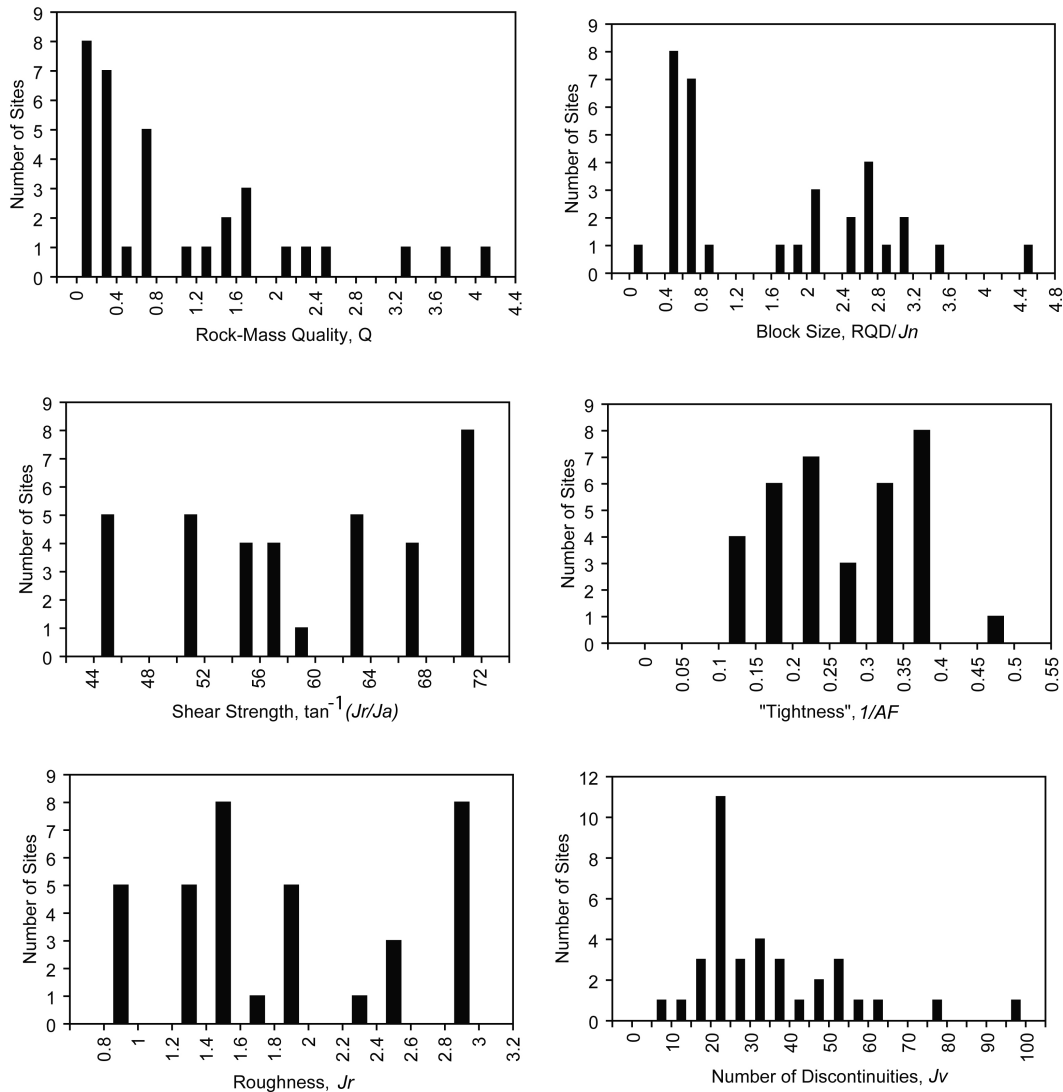
Fig. 6. Histograms showing Q and discontinuity data (see Eq. 1 in text) from the 36 Q measurement sites shown in Fig. 2. Histograms for Q , block size, and “tightness” have 2, 3, and 1, sites, respectively, with values greater than the maximum values shown on the x-axis.
