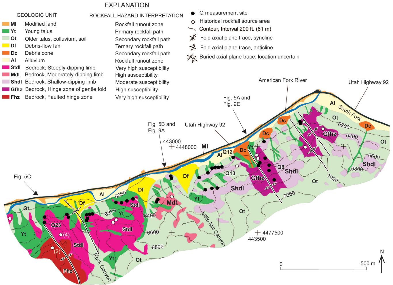
Fig. 2. Geologic map of the study area. Coordinates and tick marks are Universal Transverse Mercator, zone 12N, meters. Fold limbs are defined as follows: shallow dipping, 0–20°; moderately dipping, 20–40°; steeply-dipping, >40°. Historical rockfalls are approximately located. Numbers by two rockfalls refer to minimum quantities of falls at those locations.
