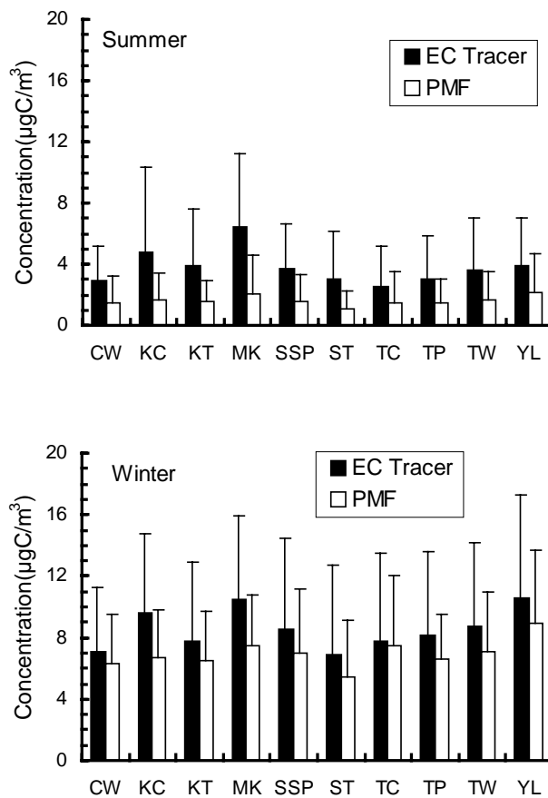
Fig. 3. Comparison of SOC estimates by the EC tracer method and by the PMF method.
