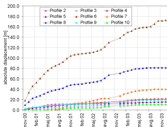
Fig. 5. Absolute displacements in measuring cross sections on the Macesnik landslide (see Fig. 3 for the position of cross sections).
