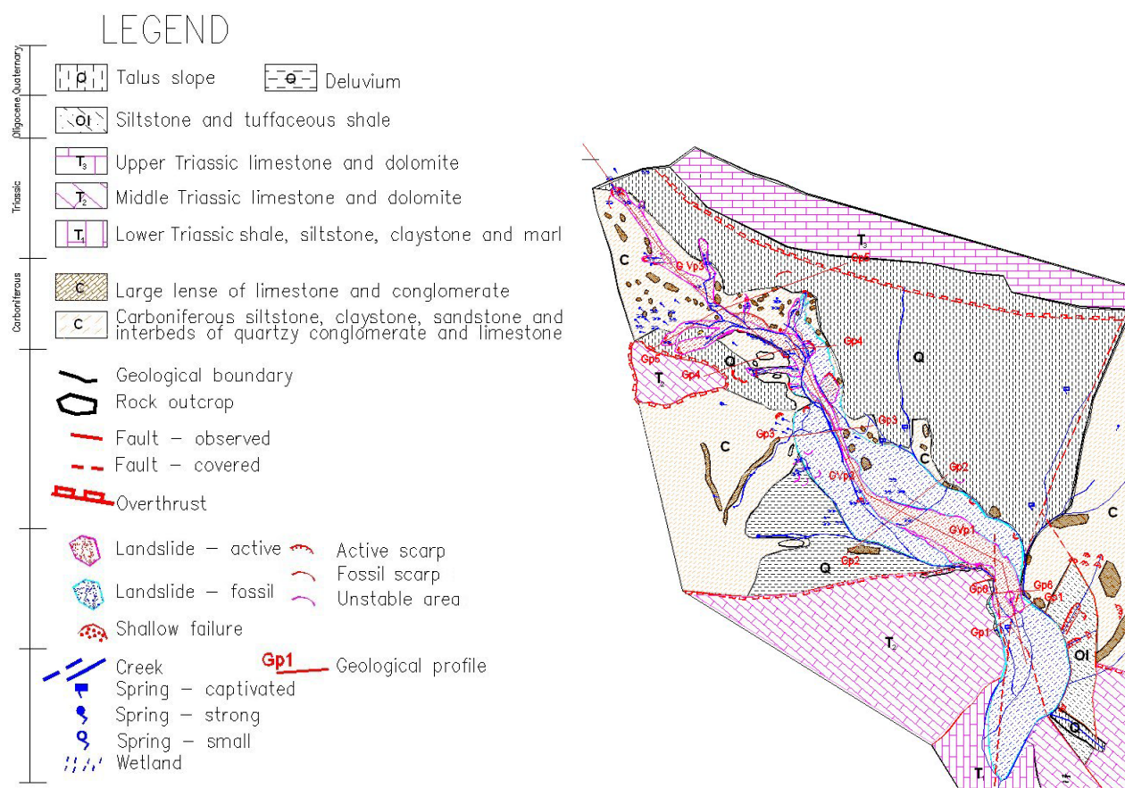
Fig. 6. Engineering geological map of the Macesnik landslide with a legend (modified from Vlaj and Žigman, 2001).
