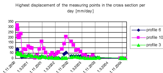
Fig. 4. Time distribution of the surface displacements of the Macesnik landslide in the period 2000–2004 in three cross sections (profile 6 – in the upper part of the landslide, profile 10 – in the area of the pontoon bridge, and profile 3 – in the area of the turn on the panoramic road).
