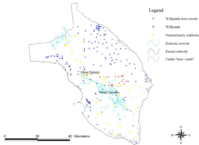
Fig. 4. Location of karstic sinkholes, wellpoints and main drainage canals.
