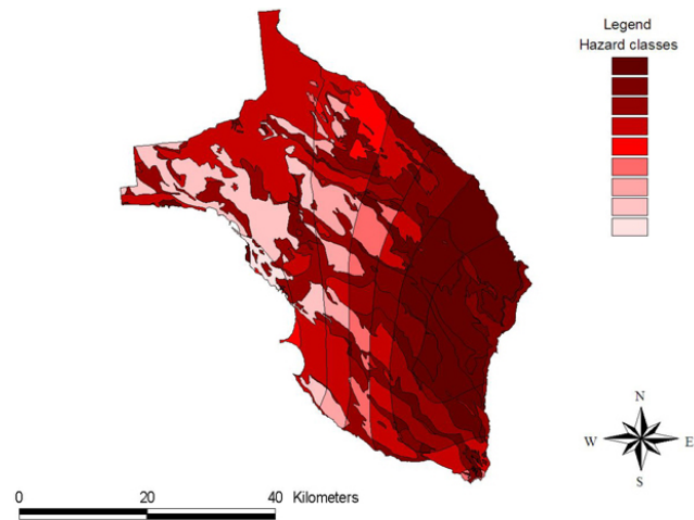
Fig. 11. Hazard flood map of Salento peninsula.
