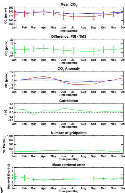
Fig. 6. As Fig. 5 but for the (a) Western Europe (left) and (b) Gobi Desert (right) regions for the year 2003.
