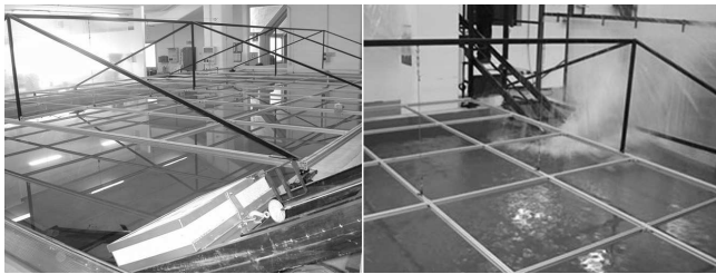
Fig. 2. Pictures from the three dimensional physical model. On the left, solid block landslide model and wave tank. On the right, impact of the landslide model with water.
