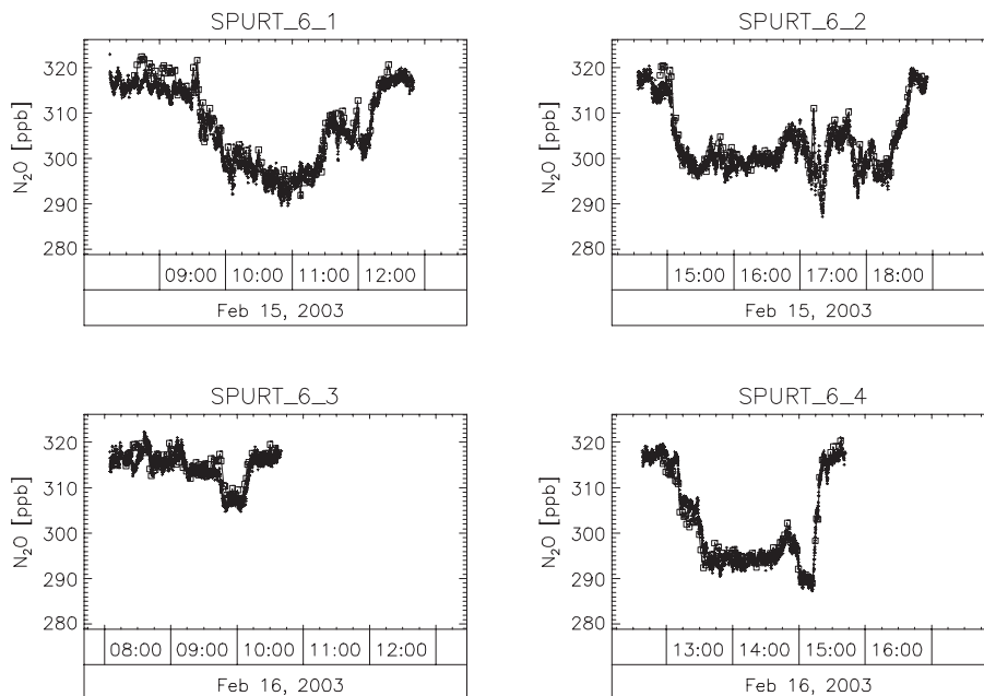
Fig. 2. Direct intercomparison of N_2O time series measured by GhOST II (open squares) and by TRISTAR (points). Due to the much higher sampling frequency, the TDL data set is much larger than the GC data. However, also small scale features are well captured by both instruments, e.g. the spike in the data observed during flight SPURT6.2 around 17:10 UTC.
