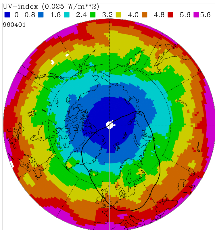
Fig. 3. UV-index on 1 April 1996. Black contour marks vortex edge.
