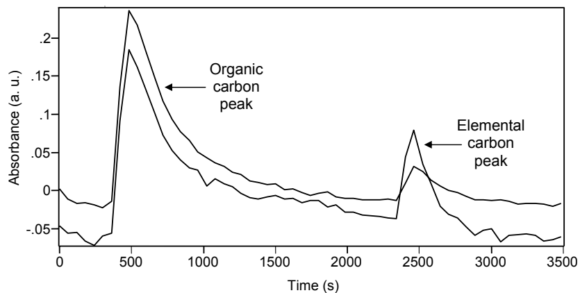
Fig. 2. CECs (CO 2 Evolution Curves) obtained by TGA/FT-IR analyzing standard b and c (a) and two particulate matter samples deposited on quartz fiber filters (b); the peaks due to organic carbon (OC) and elemental carbon (EC) are indicated with arrows.
