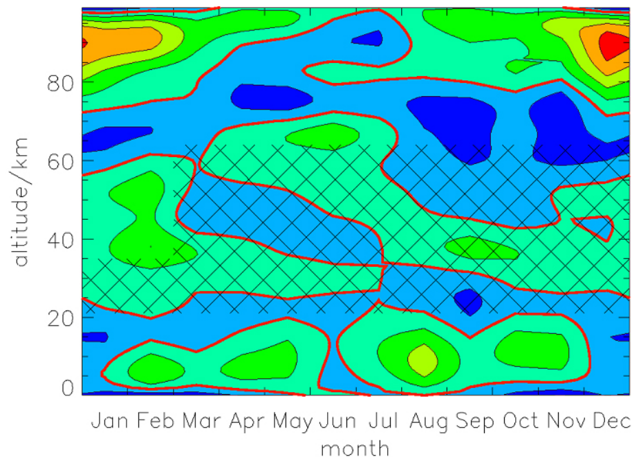
Fig. 7. Rothera zonal wind climatology (see Fig. 5) minus the HWM-93 model zonal winds. Hatched area and solid red line as in Fig. 6, contours are drawn at 5 \text{ ms}^{-1} intervals (blue: negative).
