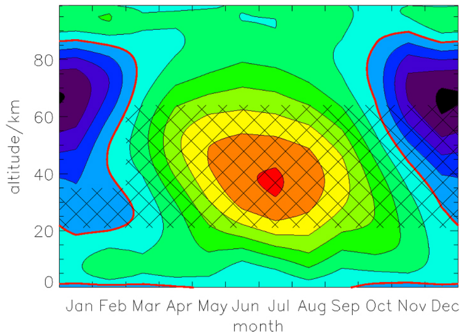
Fig. 6. Mean zonal wind above Rothera from 0–100 km. Generated from 6th order polynomial fits to the monthly mean data and, within the hatched area, monthly mean HWM-93 model winds. The thick red line represents the 0 ms -1 contour, other contours are drawn at 10 ms -1 intervals (blue: westwards).
