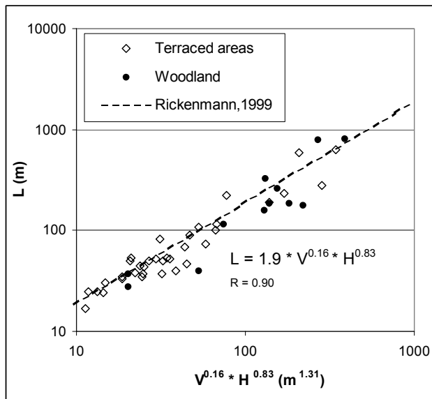
Fig. 8. Relationship among landslide total length ( L ), fall height ( H ) and volume ( V ) for the November 2000 soil slips-debris flows. Two landslide groups are used according to the different settings (terraced and woodland areas). Dashed line shows the empirical relationship proposed by Rickenmann (1999). The regression coefficient, R , has been determined considering the whole data. The exponent for the measure unit on the abscissas axis derives from Rickenmann analysis.
