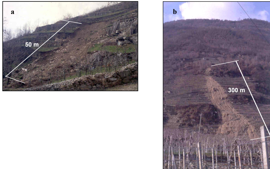
Fig. 7. Landslides on terraced areas. (a) Soil slip evolved in a small debris flow (about 50 m length) along a terraced slope; (b) the widening (up to 60 m) of an initial small soil slip (10 m wide) is shown (total length about 300 m).
