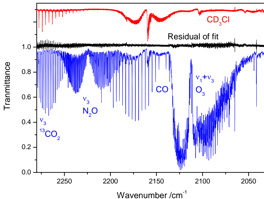
Fig. 8. FT-IR spectrum of the CD stretching region of a \text{CH}_3\text{Cl} and \text{CD}_3\text{Cl} mixture during reaction with OH radicals. The spectrum was analyzed in terms of \text{CO}_2 , CO, \text{N}_2\text{O} , \text{H}_2\text{O} and \text{O}_3 reference spectra from the HITRAN database and of the shown high resolution reference spectrum of \text{CD}_3\text{Cl} , which has been shifted for the sake of clarity.
