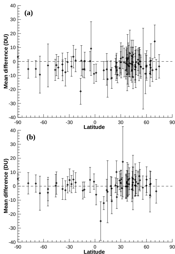
Fig. 1. Means (diamonds) and 1 \sigma standard deviations (error bars) of the Dobson minus TOMS differences at each Dobson spectrophotometer station; (a) Dobson-N7T differences (b) Dobson-EPT differences.
