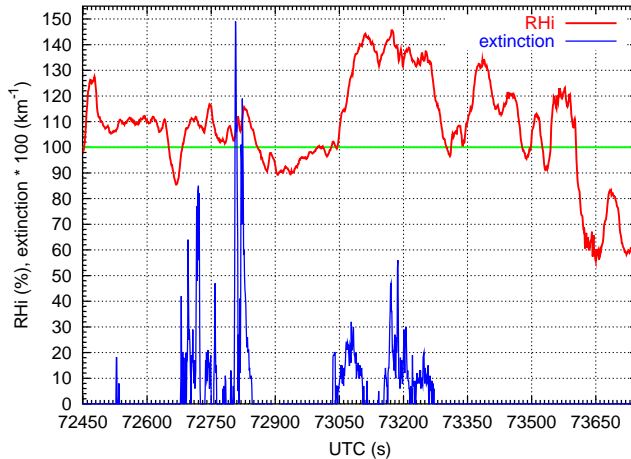
Fig. 11. Time series measurements of RH_i (in %, red curve) and extinction (in \text{km}^{-1} , scaled by 100, blue curve) along a research flight of 3 April 2000 during the INCA campaign over Punta Arenas, Chile (see e.g. Ovarlez, 2002; Gayet, 1997). Ice saturation is marked by the green line. The time resolution of the data is one second. The data show how cirrus clouds are embedded in the ISSR that extends over almost the whole flight segment (pressure \approx 286 hPa). Note also the clear but supersaturated portions.
