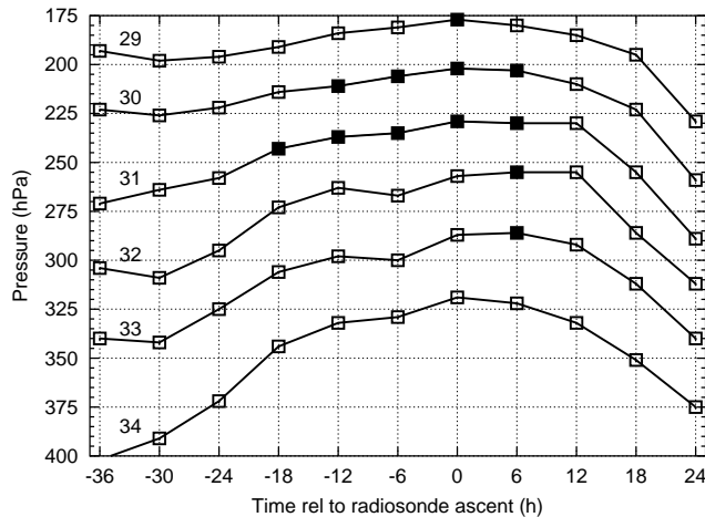
Fig. 7. Formation and evolution of the ISSR (filled square) along the main trajectories Tr_{29,1} – Tr_{34,1} (lines with open squares). The time is shown relatively to the radiosonde ascent at 29 November 2000, 06:00 UTC.
