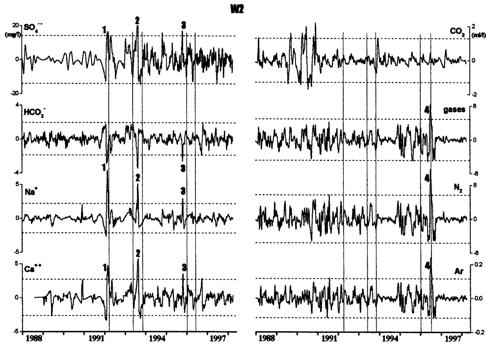
Fig. 2. Filtered and smoothed time-series of ion and gas content at W 2 from 1 January 1988 to 31 March 1998. In the plots, 1–4 represent the successes; the horizontal dotted lines represent the 3σ level. The vertical lines represent the occurrence of the five earthquakes of Fig. 1.
