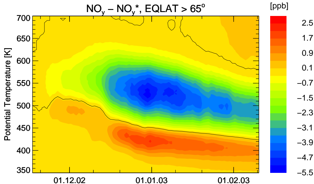
Fig. 1. Simulated redistribution of \text{NO}_y as function of time and potential temperature. Shown is the average over equivalent latitude range 65–90° N for the period 17 November 2002 to 10 February 2003. The zero contour is displayed as a black line.
