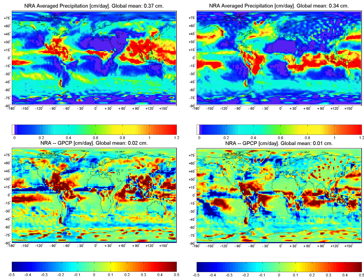
Fig. 14. Same as Fig. 13 but for NRA results in comparison to GPCP.
