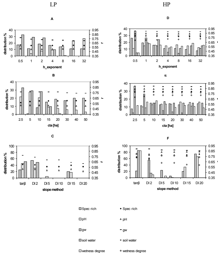
Fig. 3. Distribution of the best 10% calculation methods (bars) among different values of h , slope, and cta, as well as the highest correlation coefficient (HC) obtained using a certain parameter value (symbol) for each measured variable. (A) The h exponent parameter in the LP site. (B) The cta parameter in the LP site. (C) The slope parameter in the LP site. (D) The h exponent parameter in the HP site. (E) The cta parameter in the LP site. (F) The slope parameter in the LP site. Note the different scale on the distribution axis for slope method.
