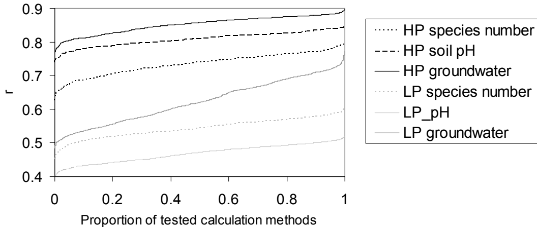
Fig. 2. Accumulated distribution of correlation coefficients obtained by using the 2688 different TWI values.
