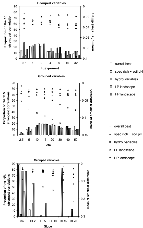
Fig. 4. Distribution of the best 10% calculation methods (bars) among different values of h , cta , and slope for different groups of measured variables. Also shown is the mean (symbol) of the smallest differences between the highest correlation coefficient and all other correlation coefficients in each group of measured variables.
