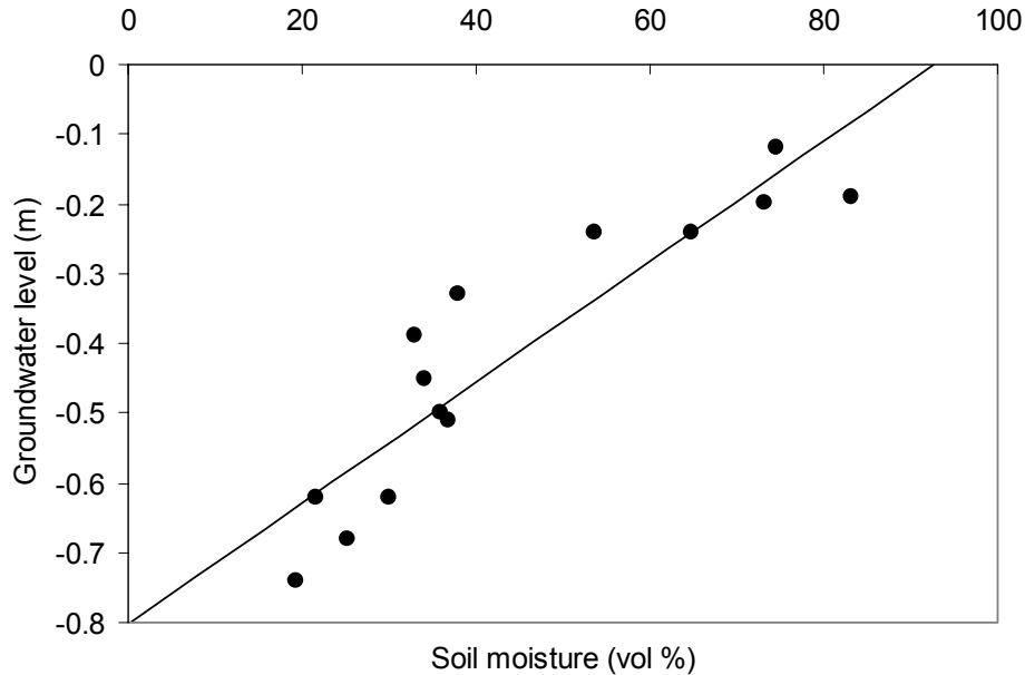
Fig. 1. Relationship between soil moisture (measured with TDR) and groundwater level at the HP site in July 2002. Both variables were measured for 14 plots ( R^2=0.823 , P>0.001 , n=14 ).
