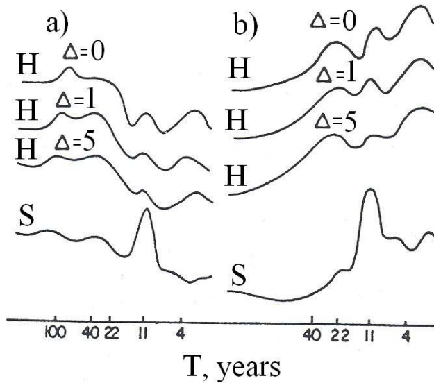
Fig. 2. Power spectra for solar activity S and water level of Lake Tchudskoye H without shift ( \Delta=0 ) and with shifts ( \Delta=1 , \Delta=5 ) between the sets of data series: (a) for the original series; (b) for the series filtered by means of the First Differences filter.
