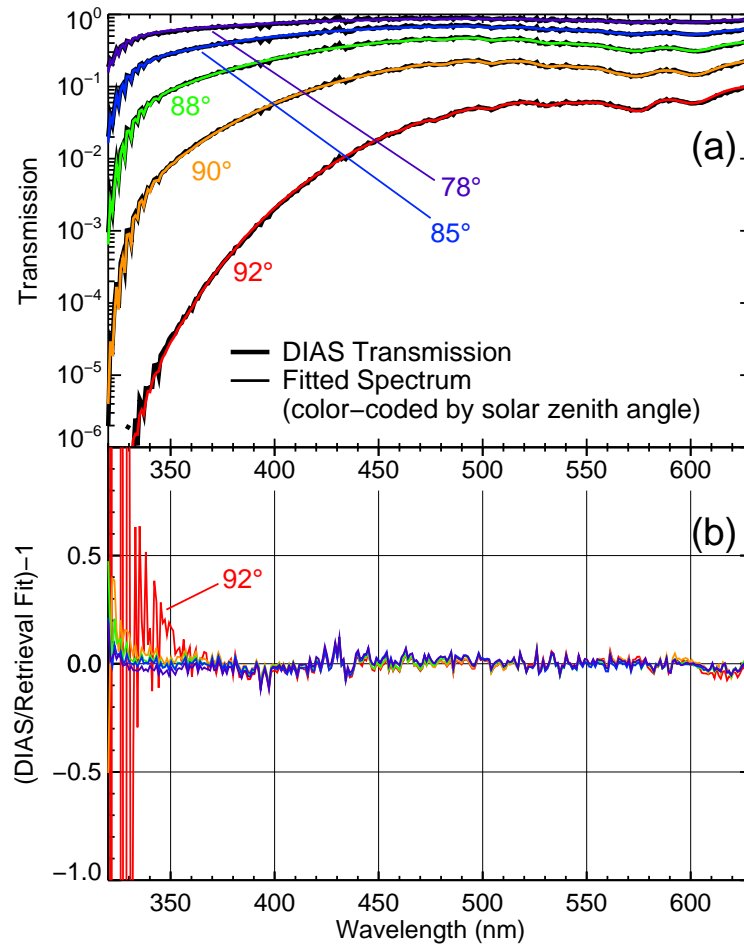
Fig. 3. Goodness of fits. (a) DIAS transmission spectra at five SZAs, 78^{\circ} – 92^{\circ} , from 6 February 2003 DC-8 flight, with fitted spectra overlaid. (b) Relative transmission difference, (DIAS/fitted spectra) – 1, with the same SZA color-coding as (a).
