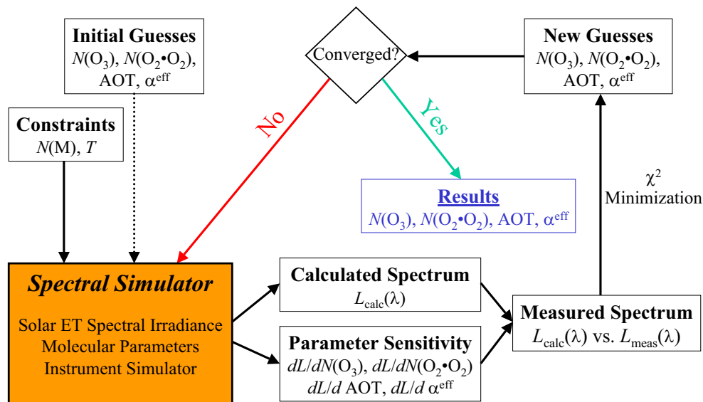
Fig. 2. Flow chart showing the algorithmic steps taken to retrieve line-of-sight composition. In this particular case, \text{O}_3 , \text{O}_2\text{-O}_2 , and the aerosol optical thickness and effective Ångström exponent \alpha^{\text{eff}} are the free parameters to be fit. The process begins with spectral simulation, based on initial guesses (which need not be accurate) of the quantities to be retrieved, geophysical constraints, and instrument spectral simulation. The calculated spectrum is compared with the actual measured spectrum, and the free parameters are adjusted. Standard \chi^2 minimization of the non-linear least squares fit is used to achieve convergence of the retrieval parameters. N() denote LOS column abundances of the indicated species, including total density N(M) ; T is the temperature; and L_{\text{calc}} and L_{\text{meas}} are the calculated and measured spectral irradiance, respectively.
