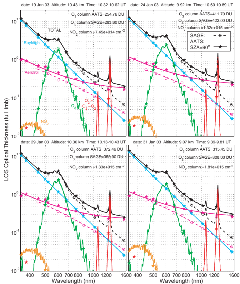
Fig. 14. Comparison of AATS and SAGE LOSOT (total and components) for 19, 24, 29, and 31 January 2003. AATS values have been converted to apparent SZA=90°, using the procedure described in Sect. 4 and illustrated in Fig. 12.
