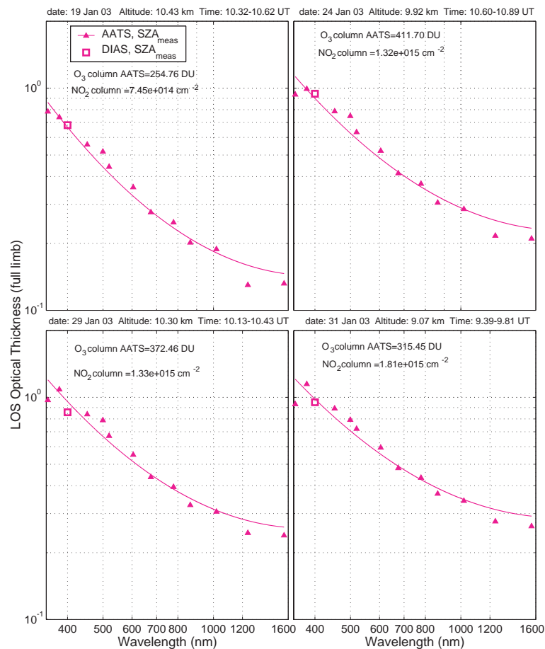
Fig. 16. DIAS LOS aerosol optical thickness (AOT) at SZA_{meas} compared to AATS LOS AOT at SZA_{meas} for 19, 24, 29, and 31 January 2003.
